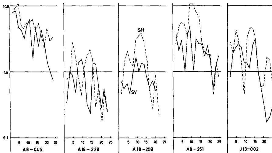
b) SV-radial and SH components of earthquakes of group I.
