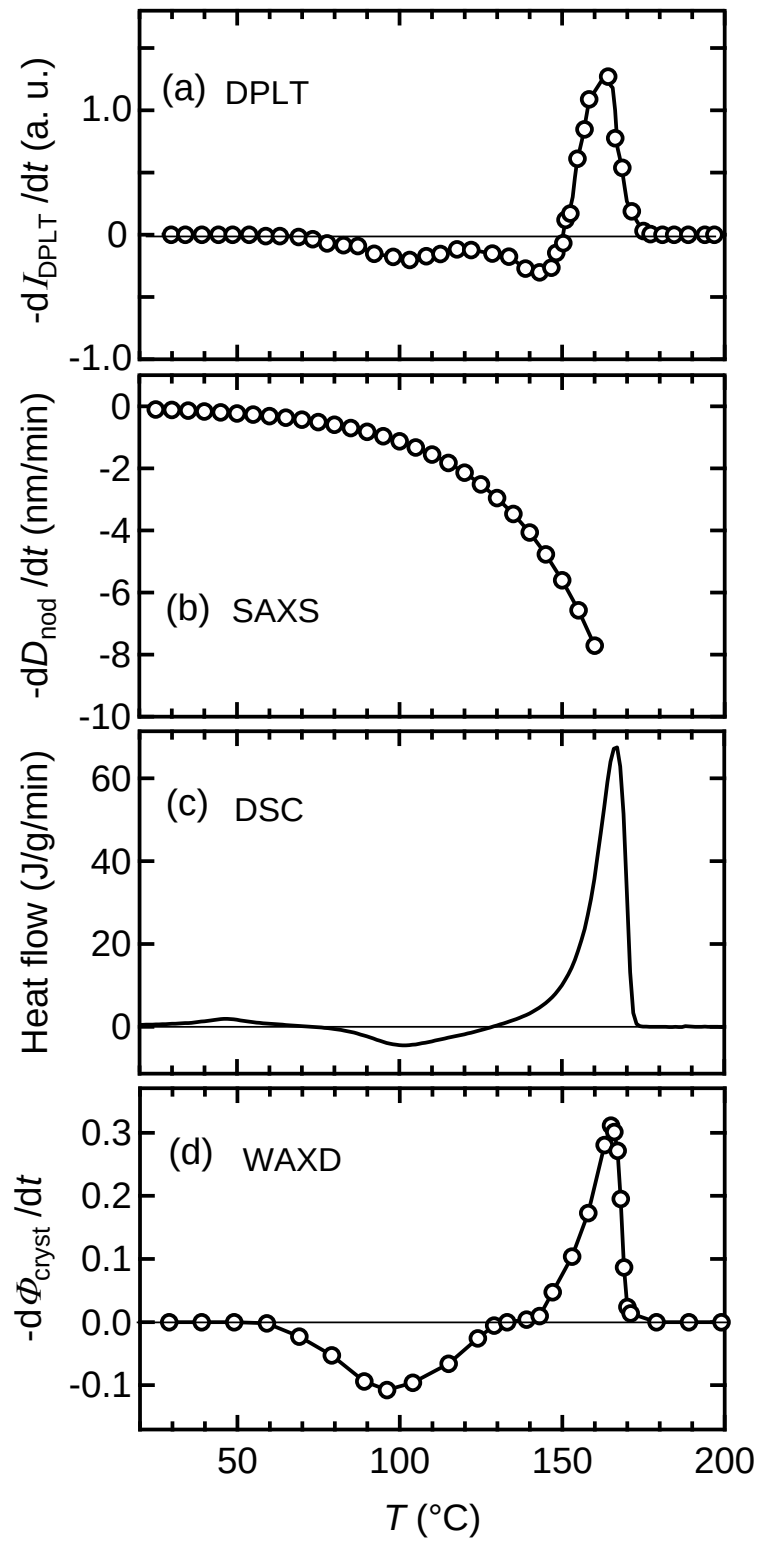
Figure 5.4. Methods-weighted rates of structure formations at a rate of 10 ^{\circ}\text{C}/\text{min} ; parts (a), (b), (c), and (d) corresponds to the methods of DPLT, SAXS, DSC, and WAXD, respectively.
