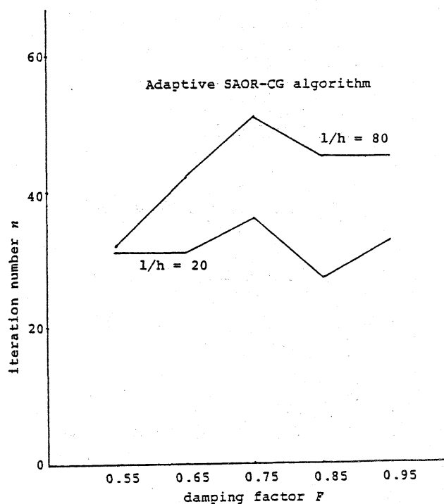
Figure 5. Effectiveness of damping factor in the Adaptive SAOR-CG algorithm.
