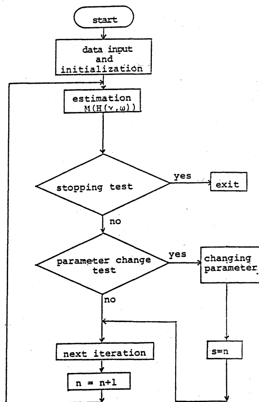
Figure 3. Flowchart of Adaptive SAOR-CG algorithm.
