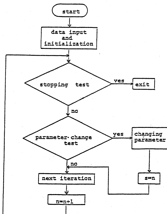
Figure 2. Flowchart of Partial-Adaptive SAOR-SI algorithm.
