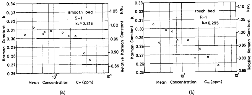
Fig. 3-11. Relation between Karman constant \kappa and mean concentration C_m . (a): smooth bed. (b): rough bed.
