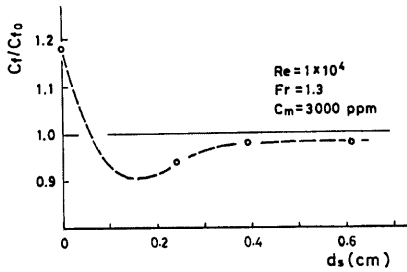
Fig. 3-6. Dependence of resistance coefficient ratio C_f/C_{f0} on bed roughness height ds .
