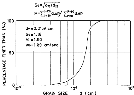
Fig. 2-2. Size frequency distribution of used sand.
