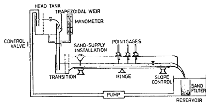
Fig. 2-1. Experimental channel.
