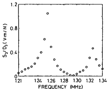
Fig. 3.16. (a), (b) Frequency characteristics of S_3 / D_3 near the first antiresonance ( about 1.3 MHz ) of the thickness-extensional mode measured at the positions (a) r = 0 and (b) r \approx 0.9R of the sample surface in the z -direction, respectively.
