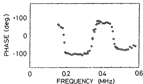
Fig. 3.19. (a),(b) Frequency characteristics of the phase of the acoustic vibration measured at the positions (a) r = 0 of the sample surface in the z -direction and (b) r = R , the edge of the sample, in the r -direction.
