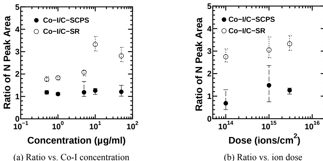
Fig. 4.10 Ratio of N peak areas between the implanted and unimplanted regions for the \text{C}^- -implanted surfaces of SCPS and SR after 2-h dipping in Co-I solution as a function of: (a) Co-I concentration at implantation condition of 10 keV and 3 \times 10^{15} \text{ ions/cm}^2 and (b) ion dose at Co-I concentration of 10 \mu\text{g/ml} .
