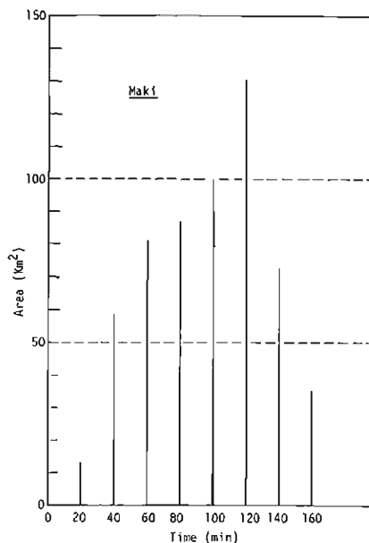
Fig. 24. The modified time-area-concentration diagram at Maki.
