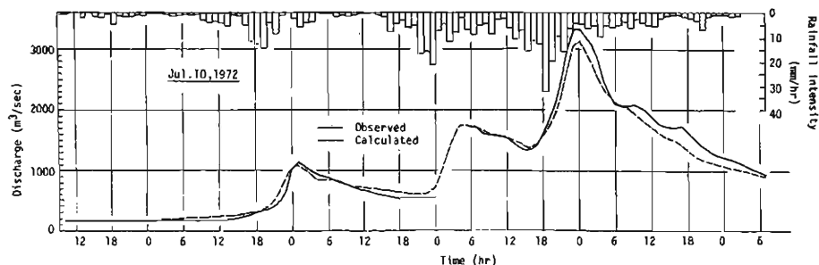
Fig. 13. Computational example of flood hydrograph at Mino in River Nagara.
