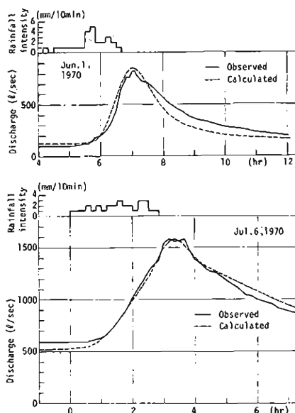
Fig. 4. Hydrographs calculated by convolution integral of the outflow from the Umegatani sub-basin and the modified time-area-concentration diagram.
