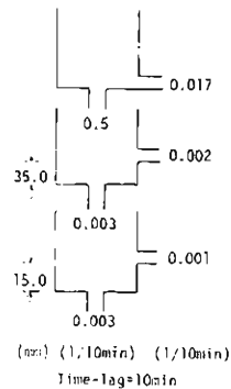
Fig. 6. The tank model used in the runoff calculation in the Umegatani sub-basin.
