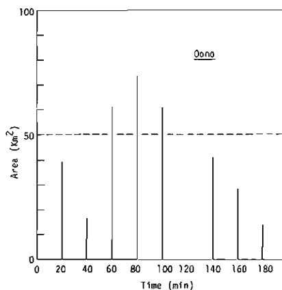
Fig. 16. The modified time-area-concentration diagram at Oono.
