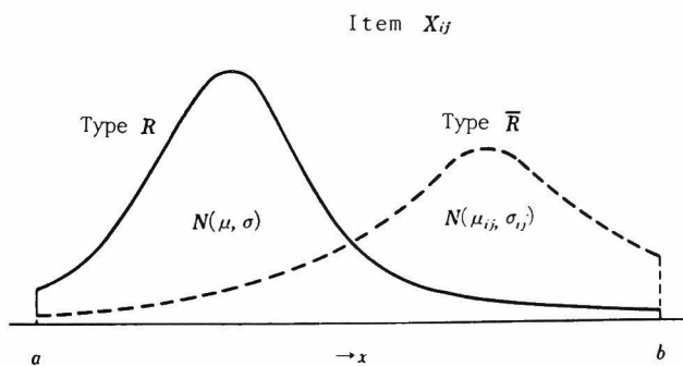
Fig. 3.4.8. Example model for computer simulation.
