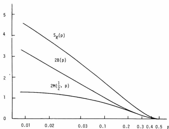
Fig. 3.3.5. The values of mean information intensity S_R and its components Bhattacharyya distance B and Shannon's mutual information M .
