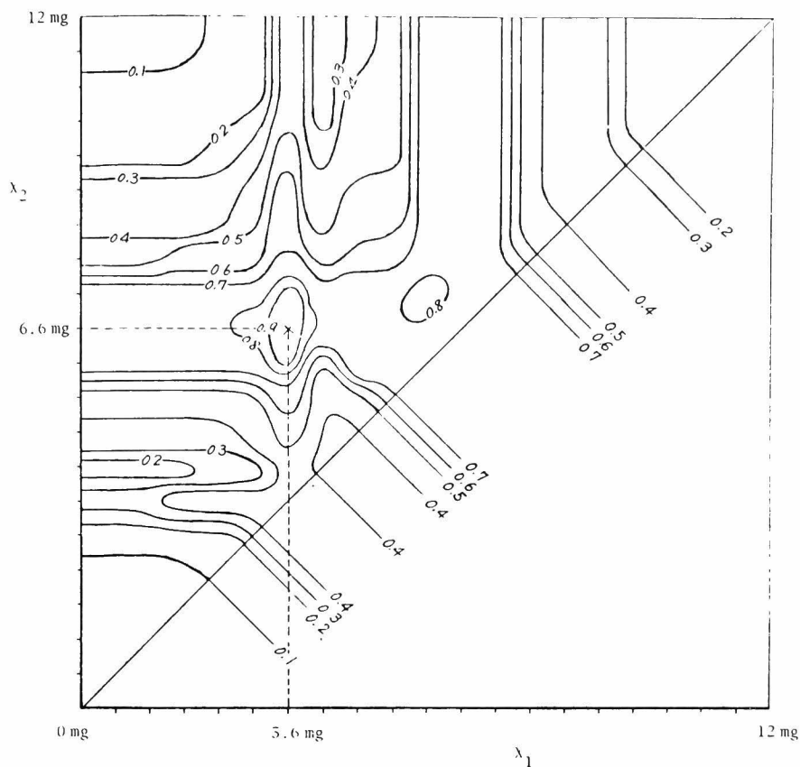
Fig. 3.4.7. The value of mean information intensity for renal failure in uric acid under three-level quantization by points x_1 and x_2 , whose maximum is attained by x_1 = 3.6 mg and x_2 = 6.6 mg.
