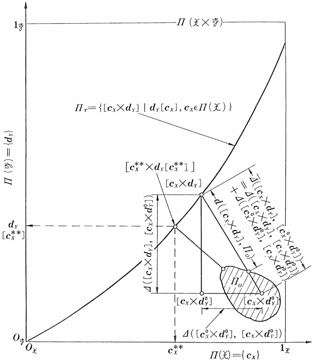
Fig. 3.4.4. Determination of suboptimum compression c_X^{**} of input information.
