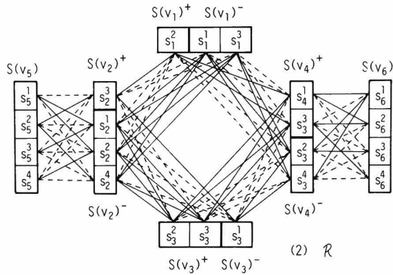
Fig. 5.4.11. An example of a totally balanced group \mathcal{R} (shown in (1)) such that its graph structure G(\mathcal{R}) contains just one circuit composed of four members v_1, v_2, v_3 and v_4 . From Theorem 5.4.11, the internal state sets S(v_1), S(v_2), S(v_3) , and S(v_4) can be partitioned as illustrated in (2), where k_i = i for i = 1, 2, 3, 4 and q = 2 (cf. equations (5.4.82) and (5.4.83)).
