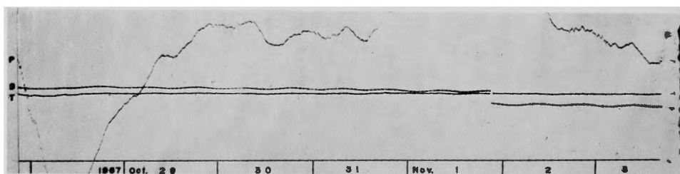
Fig. 5. Record of the ground tilt in the time of the Typhoon No. 34 on October 28, 1967.
