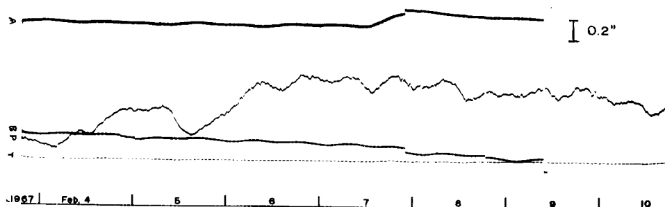
Fig. 6. A tiltgram before and after the occurrence of the earthquake on February 8th, 1967.
