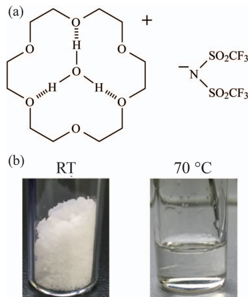
Figure 1. (a) Schematic structure of [\text{H}_3\text{O}^+ \cdot 18\text{C6}]\text{Tf}_2\text{N} and (b) Photographs of [\text{H}_3\text{O}^+ \cdot 18\text{C6}]\text{Tf}_2\text{N} at RT and 70^\circ\text{C} .
