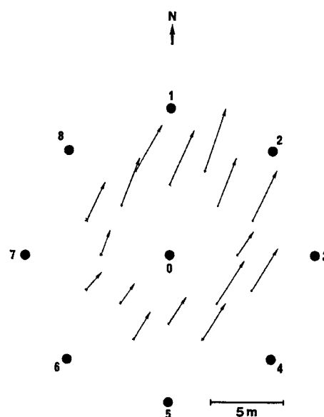
Fig. 12. An example of spatial distribution of the preferred orientation angles of leaked currents at an extremely local place.
