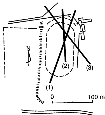
Fig. 5. Schematic position of the Obaku fault lines proposed by Irikura et al. 6) (1), Kobayashi et al. 5) (2) and Mino et al. 7) (3).
