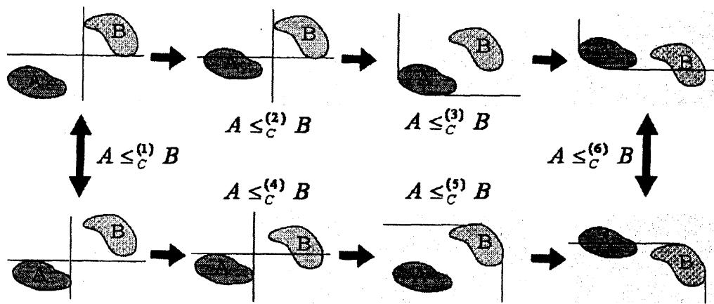
Figure 1. Six kinds of classification for set-relationship.
