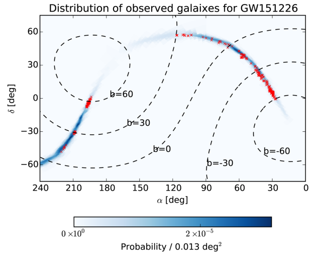
Fig. 3. Positions of the galaxies observed in the J-GEM follow-up observation of GW151226 (red points). (Color online)
