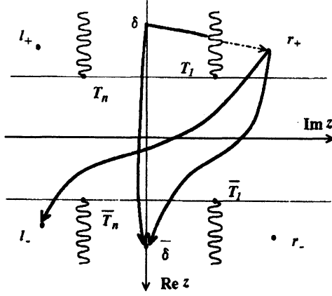
Figure 7: n \geq 2 , \operatorname{Re} z(T_n) = \operatorname{Re} z(T_1)
