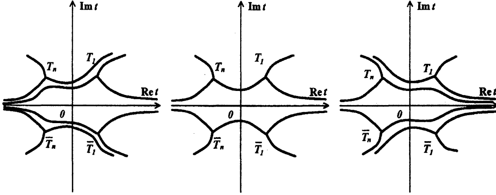
Figure 4: \operatorname{Re} z(T_n, T_l) < 0 Figure 5: \operatorname{Re} z(T_n, T_l) = 0 Figure 6: \operatorname{Re} z(T_n, T_l) > 0
