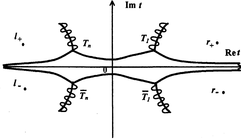
Figure 2: symbol base points
