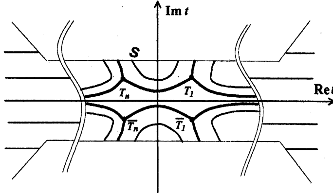
Figure 1: Stokes geometry
