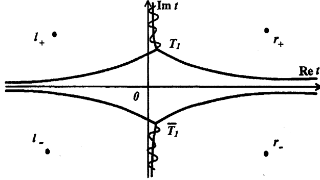
Figure 3: Stokes geometry n = 1
