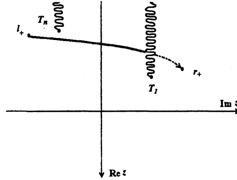
Figure 9: n \geq 2 , \operatorname{Re} z(T_n) < \operatorname{Re} z(T_1)
