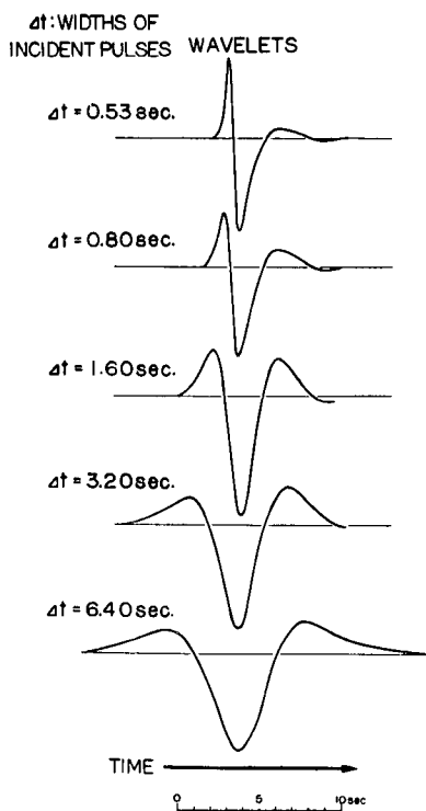
Fig. 5 Theoretical seismograms against Knopoff's displacement pulses.
