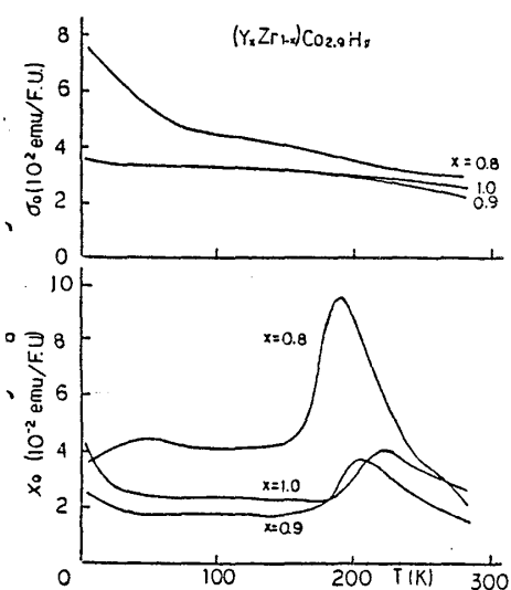
図5 (Y_xZr_{1-x})Co_{2.9} ( X \geq 0.8 )
