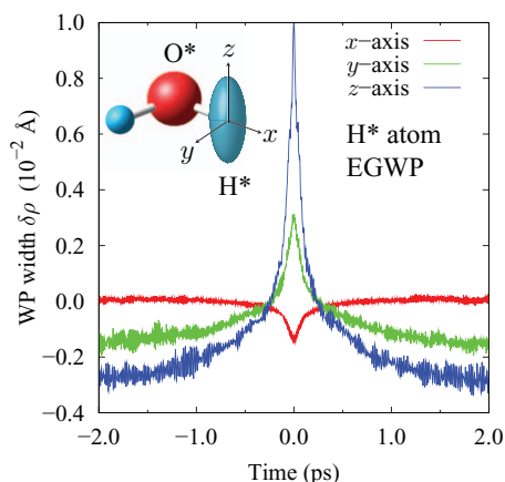
FIG. 6. Averaged H-bond exchange trajectories of the WP width fluctuations of the jumping hydrogen atom H* in the body-fixed axes obtained from the SQ simulation with the EGWP model. Also shown is the graphical definition of the body-fixed axes for the H* atom.
