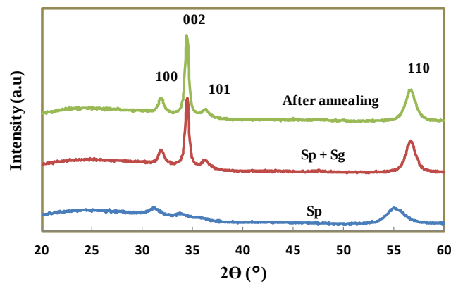
Fig. 6-2 Crystal orientation in different step of AZO film prepared by combining both sputtering and sol-gel method.
