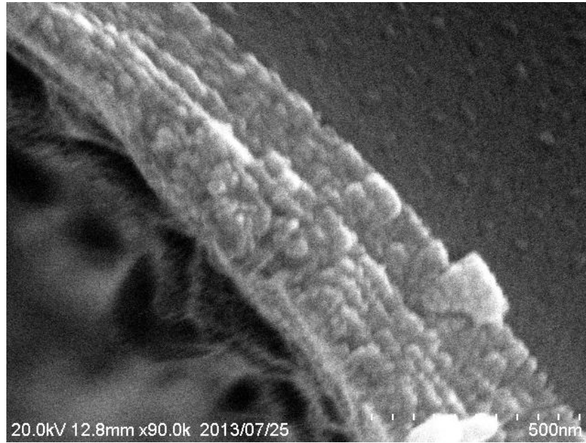
Fig. 4-7 Cross sectional view of AZO thin film
