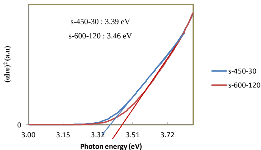
Fig. B-1 (a) Transparency curve and (b) Tauc plot
