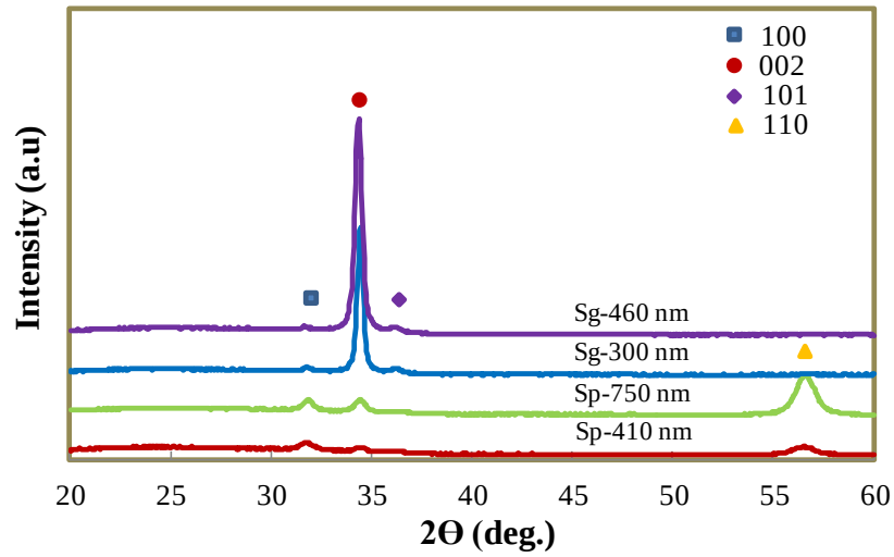
Fig. 5-3 XRD curve of AZO films. (Here, Sg and Sp indicates sol-gel and sputtering, respectively)
