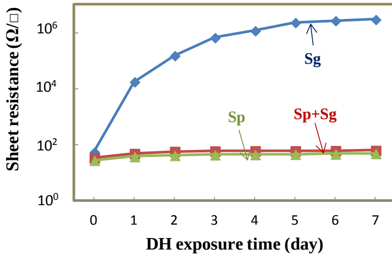
Fig. 6-4 Damp heat test result of Sg, Sp and Sp+Sg films
