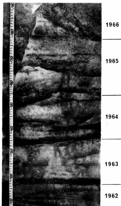
Figure 6. Part of Firn Profile in the wall of a pit at Point L/L, showing the icy layers (dark bands) and the net accumulation for successive budget years.
