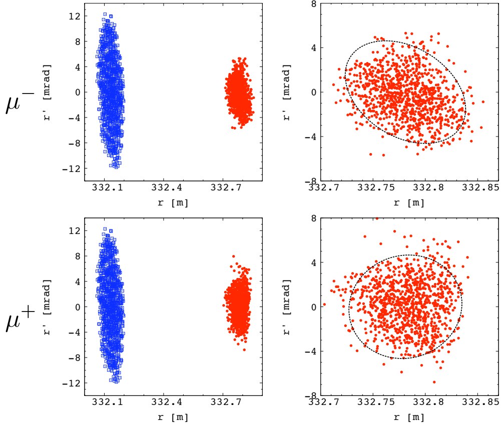
Figure 4.18: Horizontal (r, r') phase space plots showing the position of \mu^- (upper plots) and \mu^+ (lower plots) at the beginning (blue squares) and at the end (red dots) of the acceleration cycle. In the plots on the right, dotted-line ellipses are shown together with the position of particle at the end of the acceleration cycle. The area of these ellipses correspond to a emittance of 30 \pi \text{ mm.rad} normalized at 12.6 GeV. The parameters of these ellipses are chosen with respect to the periodic Twiss parameters calculated at 12.6 GeV. Here less than about 10 % of the particles are lying outside of these ellipses, which indicates a certain amount of emittance blow-up.
