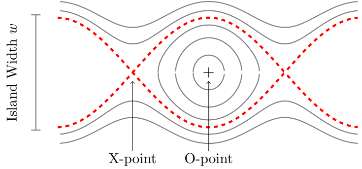
Figure 6.1: Sketch of the flux surfaces of a magnetic island. The magnetic island changes the topology of the magnetic field, with characteristics points being the O-point, X-point and the separatrix (dashed line).
