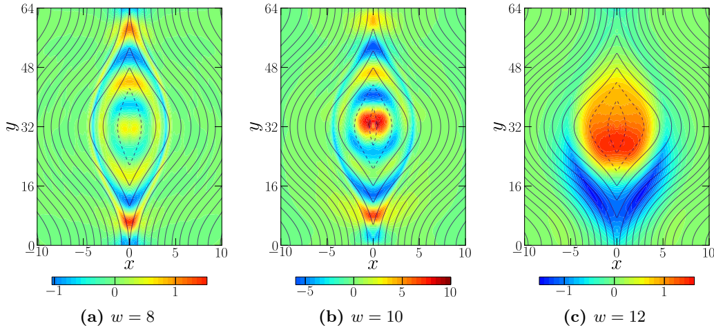
Figure 6.26.: Contour of the electrostatic potential at t = 800 for the kinetic electron case with m_{ie} = 800 , \eta_i = 5 and a finite electron temperature gradient of \eta_e = 2 . In contrast to the isothermal electron case, a strong vortex mode is not found for moderate island widths up to w \leq 10 . Showing that a finite electron temperature gradient also has a large influence on the dynamics.
