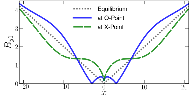
Figure 6.13: Perturbation of the equilibrium field due to the magnetic island at the X- and O-point, i.e., y_X = 0 and y_O = L_y/2 , respectively. The rational surface formation at the O-point is clearly visible. The field structure at the X-point has a strong increase in magnetic shear.
