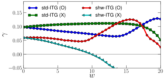
Figure 6.14: Growth rate of drift turbulence at the island's X- and O-point for k_y = 0.5 and k_y = 2.5 modes. Rational surface separation at the O-point destabilizes the std-ITG region, as well as the shw-region. The onset of destabilization for the shw-region is earlier compared to the std-region.
