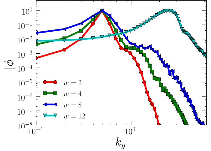
Figure 6.11: Mode spectrum of the electrostatic potential for k_y for island widths of w = 2, 4, 8, 12 . For small islands widths the mode spectra coincides with the linear peak growth rate from the standard ITG mode, for large islands, the peak of the mode spectra shifts to the peak growth rate of the short-wavelength ITG mode.
