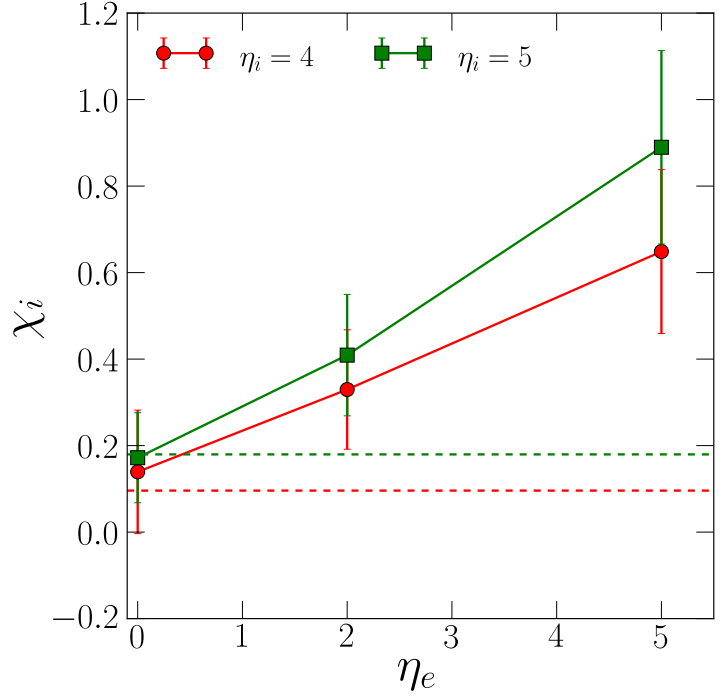
Figure 5.24: Comparison of the nonlinear heat fluxes with kinetic electrons for m_{ie} = 500 over \eta_e for the cases with \eta_i = 4 and \eta_i = 5 . The dashed lines corresponds to the adiabatic case. We find that for \eta_e = 0 , ion heat fluxes are comparable to the adiabatic case. For \eta_e > 0 heat flux increases.
