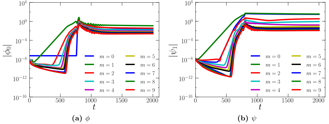
Figure 6.3.: Time evolution of the Fourier modes of \phi_0 and \psi_1 . We find that in the linear phase, the m = 1 mode is the only unstable mode. The other modes are excited nonlinearly once the evolution enters the saturation phase. At the t = 2000 , we reached the steady-state full reconnection phase.
