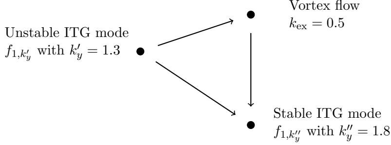
Figure 4.17.: Sketch of the mode coupling triad between the unstable mode with k'_y , the stable mode with k''_y and the tertiary mode k_{ex} .
