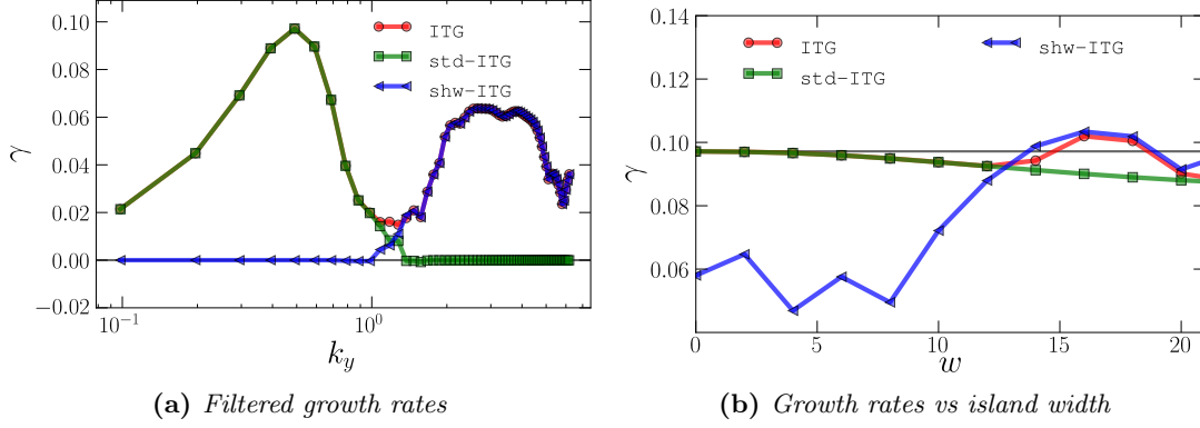
Figure 6.12.: Linear growth rates for three cases : the original case (ITG), a case with the short-wavelength part suppressed (std-ITG) and a case with the standard part suppressed (shw-ITG). Left figure shows the linear growth rates in the absence of an island. Right figure shows the growth rates with increasing island width - only when the short-wavelength part is present, a destabilization at w \sim 14 is observed (right figure).
