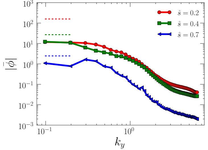
Figure 5.17: Averaged turbulence spectra (of \phi ) for the ITG between t = 1000 - 2000 . Physical parameters are \eta_i = 5 and \hat{s} = 0.2, 0.4, 0.7 . The dashed line corresponds to the zonal flow level. A high zonal flow level is found that exceeds the level of other modes. No significant peak is found where the short-wavelength modes are linearly unstable. For k_y > 3 a flattening is found which can be attributed to the remaining aliasing originating from the nonlinear term.
