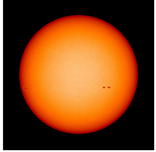
Figure 1.1: Picture of our sun in the visible spectra taken at February 28, 2013 [image credit : NASA]. The sun is a hot glowing ball of gravitational bound plasma with a surface temperature of 6000K. The energy is produced in the sun's core, where the temperature reaches up to 15.2 Million Kelvin, allowing the ions to overcome the electrostatic repulsion and the fusion of hydrogen into helium. It is estimated that the sun's fusion process has lasted for over 4.6 billion years and will continue to do so for another 5 billion years.
