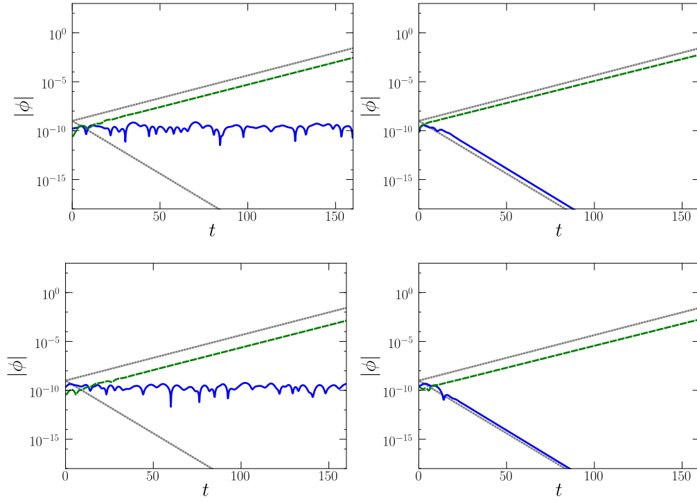
Figure 4.22.: Solution of the IVP with \epsilon = 0.15 and k'_y = 1.3 (solid) and k''_y = 1.8 (dashed), with the corresponding Landau solutions (dotted). Without coupling ( \epsilon = 0 ), the stable mode can only be resolved with large enough collision, see \beta_c = 0 (a) and \beta_c = 5 \times 10^{-3} (b). With coupling, i.e. \epsilon = 0.15 , the growth rate of the coupled global mode is independent on the collisionality, see (c) with \beta_c = 0 and (d) with \beta_c = 5 \times 10^{-3} .
