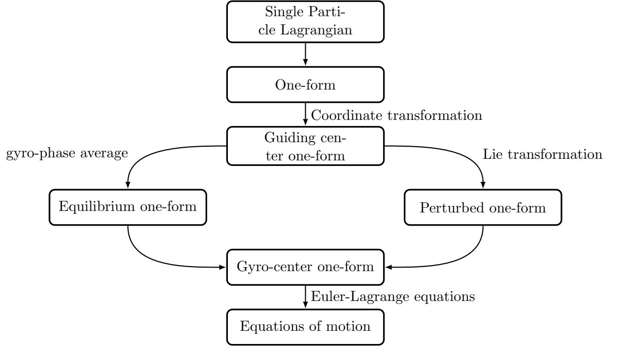
Figure 2.3.: Outline of the gyro-averaging procedure to derive the gyrokinetic Vlasov equations [adapted from Görler (2009)].
