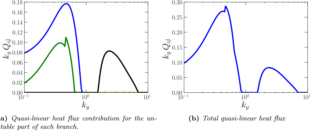
Figure 5.8.: Quasi-linear heat flux contributions of the ITG mode with \eta_i = 5 and \hat{s} = 0.2 . Left figure shows the separated contributions of each unstable part of the branches. The dominating contributions is from the dominant ITG mode. With the first sub-dominant and the short-wavelength region having are equally contributing. The sub-dominant mode shows a discontinuity due to symmetry change. Right figure shows the summed contributions per k_y , the standard region contributes majority to quasi-linear heat flux.
