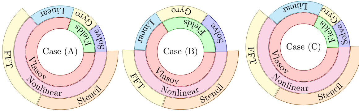
Figure 3.7.: Results of profiling of the gkc++ code for the cases (A-C) are shown in a sunburst diagram. The angle of the circle segment corresponds to the fraction of the total computational time spent. Inner layers corresponds to low hierarchy, upper layer to higher hierarchy. All cases show that the majority of the time is spent within the Vlasov solver, where roughly two thirds of the total computational time is spent on calculating nonlinearity.
