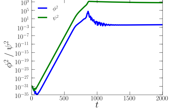
Figure 6.2: Time evolution of flow energy ( |\phi^2| ) and flux energy ( |\psi^2| ) with an unstable setup resulting in the formation of a magnetic island. Magnetic reconnection at the rational surface is self-amplifying and thus exponential growth is observed until t \sim 550 . Around t \gtrsim 550 the Rutherford regime is entered, where exponential growth is replaced by an algebraic growth. Saturation sets in at t \sim 600 and a full reconnection state is reached at t \sim 1300 . Throughout the whole evolution, we observe that the magnetic flux energy is dominating over the kinetic flow energy.
