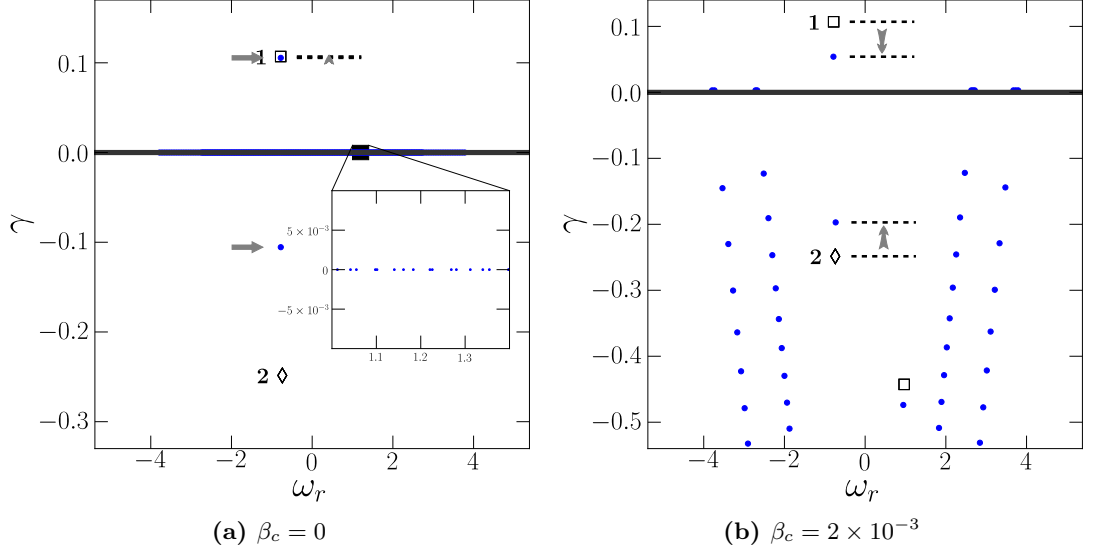
Figure 4.18.: Eigenvalue spectra of the coupled poloidal modes with k'_y = 1.3 and k''_y = 1.8 for the collisionless and weak collisional case with \epsilon = 0.15 . The Landau solutions for the uncoupled modes are shown using square markers.
