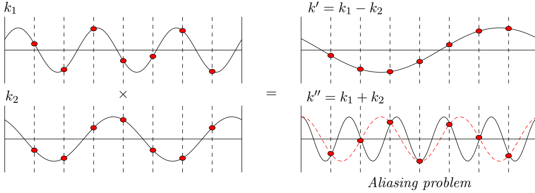
Figure 3.6.: A quadratic nonlinearity coupled both modes and produces new modes given by k = k_1 \pm k_2 . The largest frequency the grid can resolve is below the Nyquist frequency given here by k_y \max = N_y/2 . If a nonlinearity produces wave above the Nyquist frequency the grid cannot resolve it anymore and it gets mapped back, here, k'_y = 3 - 2 = 1 and k''_y = 3 + 2 = 5 \equiv 3 . This aliasing problem causes numerical oscillations leading to non-physical results and thus has to be avoided.
