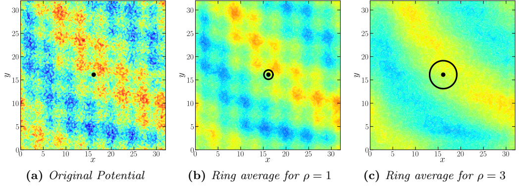
Figure 2.8.: Effect of gyro-averaging for a random potential for various gyro-radii. A smoothing effect is observed for the ring average.
