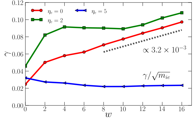
Figure 6.25: Linear growth rates of electrostatic potential vs magnetic island width for varying \eta_e using \eta_i = 5 and m_{ie} = 800 . For the case without the island, a resonance of the electrons at the rational surface reduces growth rate. For small island widths the resonance effect is reduced, such that the growth rates quickly rises. For intermediate island widths, a stabilization effect is observed for \eta_e = 2 which for a critical island width of w = 2 gets destabilized. Note that for the case of \eta_e = 5 , the ETG is excited and dominated the global mode.
