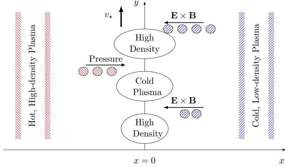
Figure 5.1.: A simplistic picture of the excitation of an temperature gradient drift mode in slab geometry through the interplay of temperature gradient and \mathbf{E} \times \mathbf{B} drift and pressure force.
