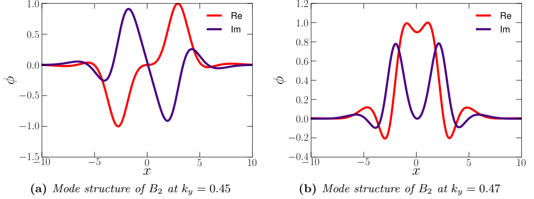
Figure 5.9.: Eigenmode structure of the first sub-dominant branch B_2 in the standard ITG region. At k_y \sim 0.5 , the eigenmode structure of the electrostatic potential changes its symmetry from an anti-symmetric mode structure (left figure) to a mirror-symmetric mode structure (right figure). This results in the discontinuity observed in the quasi-linear heat flux estimates.
