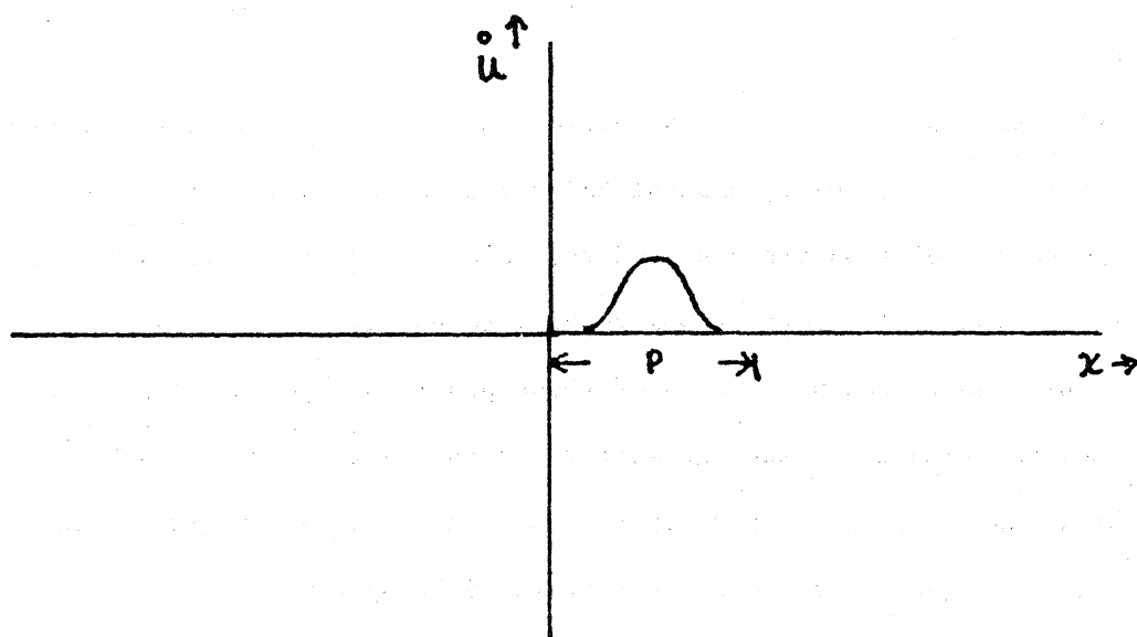
Figure I.2. One period of u(x) .
