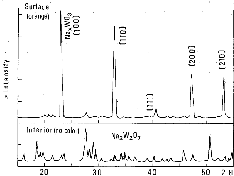
Fig. 5. X-ray diffraction of a crystallized glass having a bronze layer at the surface. Glass NWP 16 \text{Na}_2\text{O} 33.5, \text{WO}_3 65, \text{P}_2\text{O}_5 1.5
