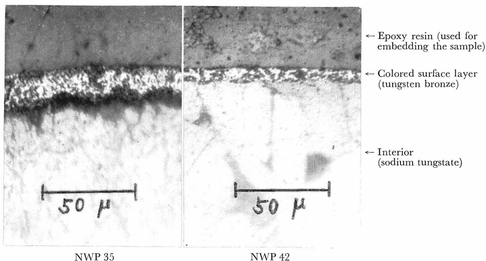
Fig. 3. Cross sections of the glass-ceramics having a tungsten bronze surface layer. See Table 1 for the compositions of the samples.
