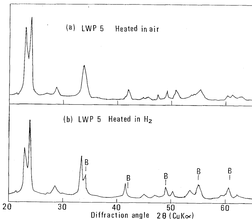
Fig. 10. X-ray diffraction patterns of a \text{Li}_2\text{O}-\text{WO}_3-\text{P}_2\text{O}_5 glass (LWP 5) after crystallization.
