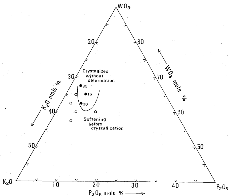
Fig. 8. \text{K}_2\text{O}-\text{WO}_3-\text{P}_2\text{O}_5 compositions used in the experiment.
