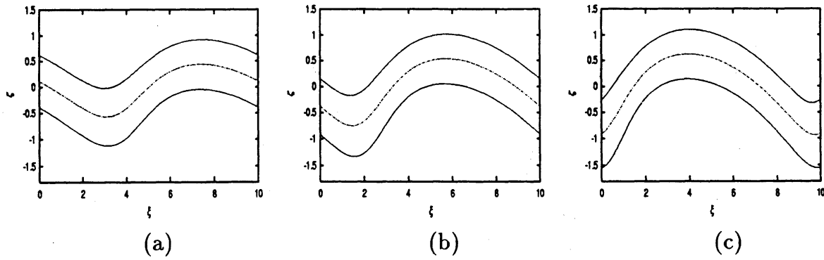
FIG 5. \Delta\Theta = 0.44 (\tau = 250) ; (a) G=0 , (b) G=0.5 , (c) G=1.0 .
