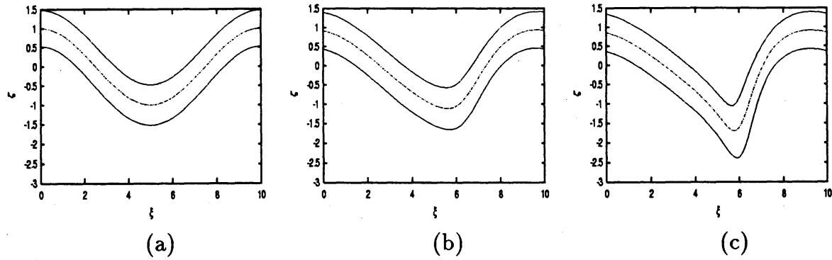
FIG 6. \Delta\Theta = 0.5 (G=0) ; (a) \tau = 0 , (b) \tau = 3.0 , (c) \tau = 6.0 .
