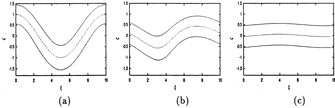
FIG 4. \Delta\Theta = 0.44 (G=0) ; (a) \tau = 0 , (b) \tau = 250 , (c) \tau = 500 .
