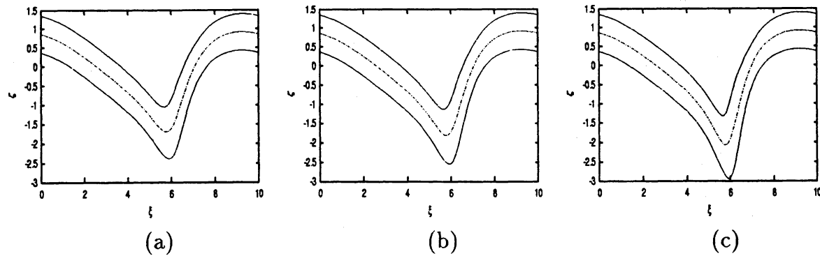
FIG 7. \Delta\Theta = 0.5 (\tau = 6) ; (a) G=0 , (b) G=0.5 , (c) G=1.0 .
