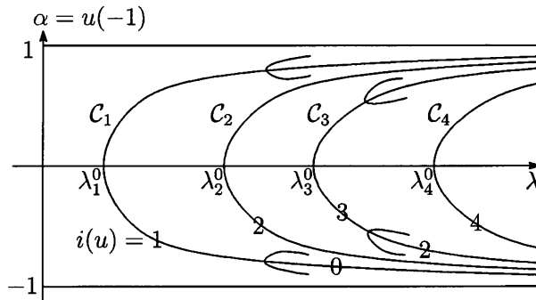
Bifurcation diagram of (1.1).
