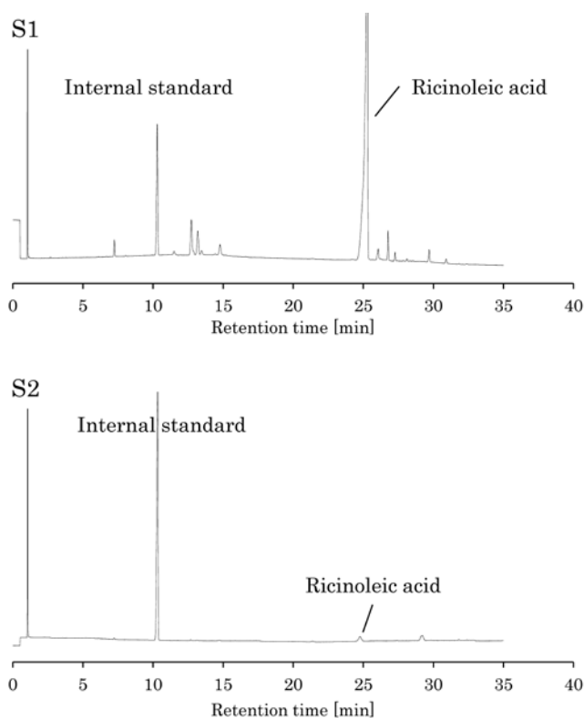
Fig. 4. GC chromatograms of methyl esterified lipids in culture medium of S1 and S2. GC methods were described in Materials and Methods.
