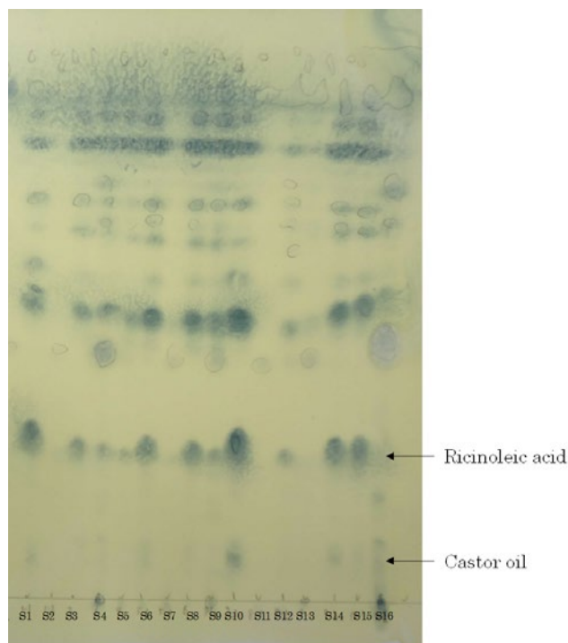
Fig. 2. TLC analysis of lipid composition in culture medium containing microorganisms isolated by the enrichment culture method. TLC methods were described in Materials and Methods.
