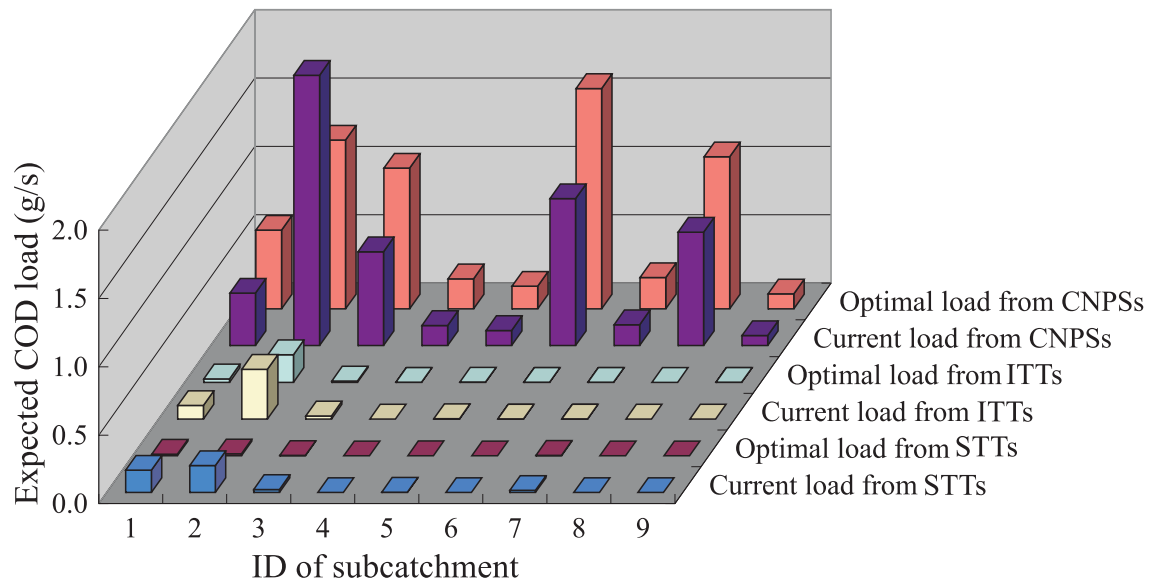
Fig. 7. Optimal COD loads allocated to CNPSs, ITTs and STTs in <Solution C>.
