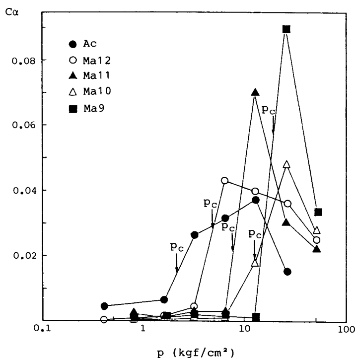
Fig. 9 Representative C_\alpha -values of marine clay strata.
