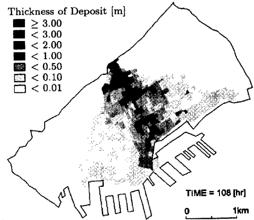
Fig. 15 Thickness of sediment deposit
