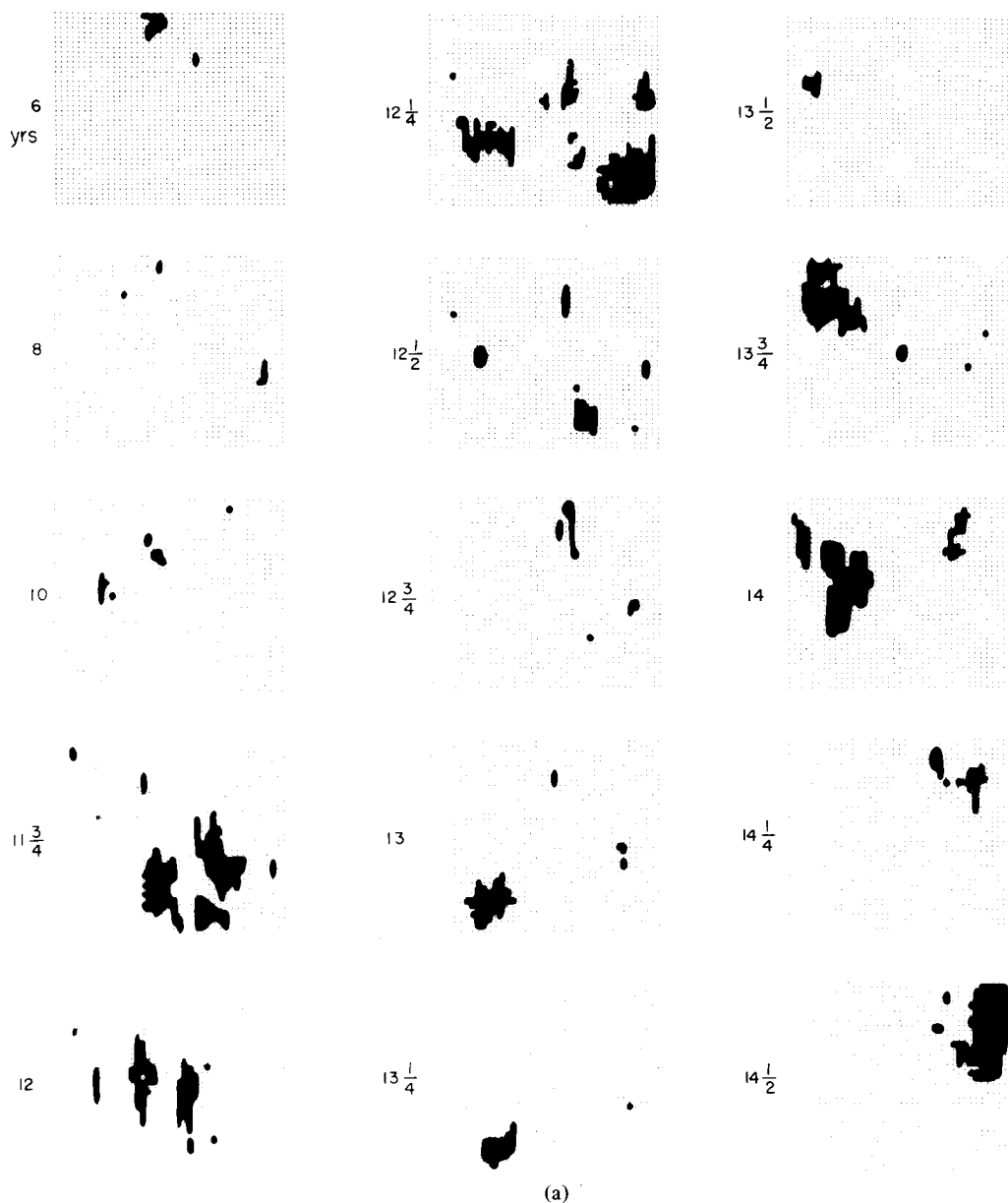
Figure 11. Space and time patterns of major shocks in the time range up to 25 yr. Time step is indicated by yr. (Case M-111 slightly modified from M-11.)
