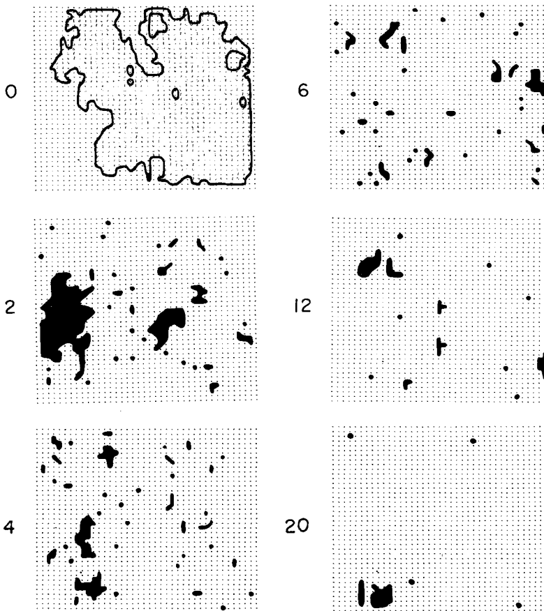
Figure 3. Space and time patterns of aftershocks for Case M-12. Numerals in the left-side of each time step indicate the elapsed time (in hr) after the main faulting. Fault dimension; 40 \times 40 km, segment size; 1 \times 1 km. (The same explanations apply to Figs 4, 5, 6 and 7.)
