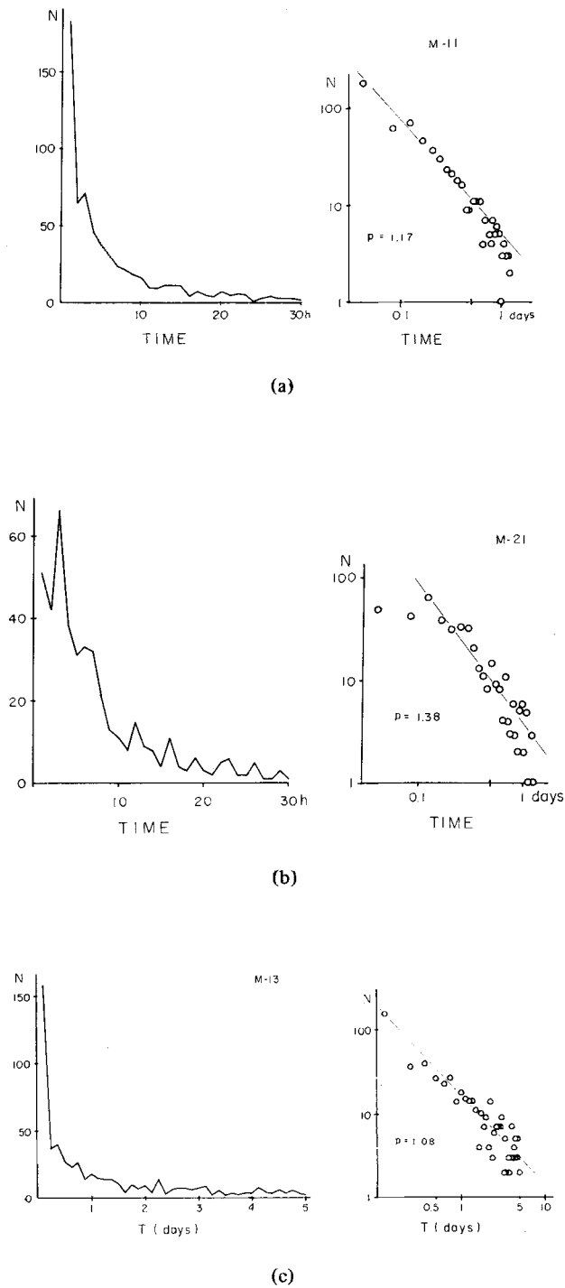
Figure 8. Frequency of aftershocks with time. Left: linear scale, right: logarithmic scale. (a) Case M-11, (b) Case M-21, (c) Case M-13.
