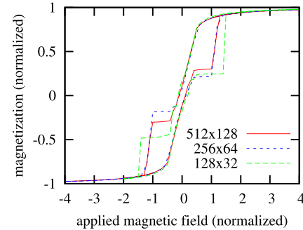
FIG. 4. Magnetization curves given by micromagnetic simulation with 128 \times 32 \times 1 , 256 \times 64 \times 1 , and 512 \times 128 \times 1 cells.
