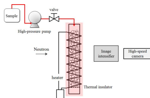
Figure 1 Schematic diagram of the apparatus
