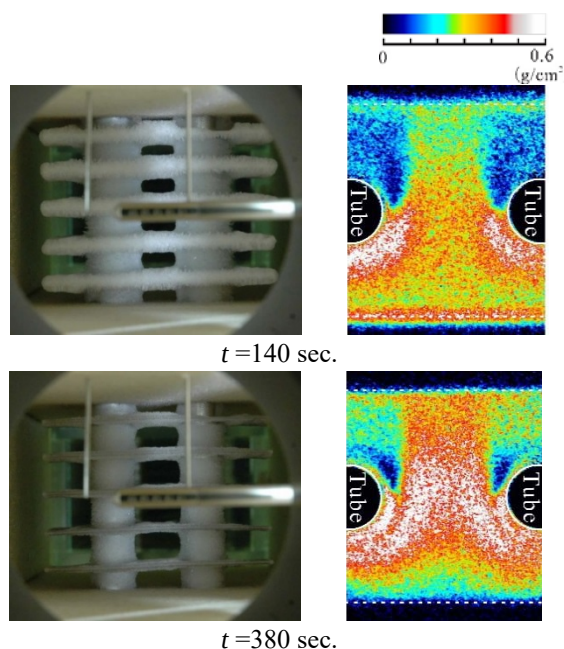
(a) Digital camera image (b) Water deposition m_w Fig.2 Water deposition profiles on the fins.
