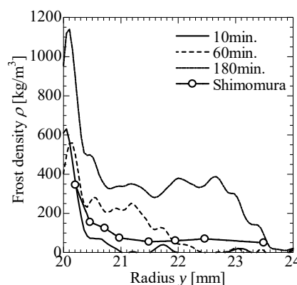
Fig.3 Distribution of frost density with height.
