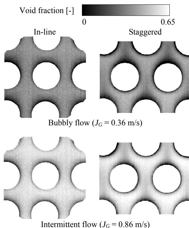
Fig. 1. Two-dimensional void-fraction distributions in in-line and staggered tube bundles.
