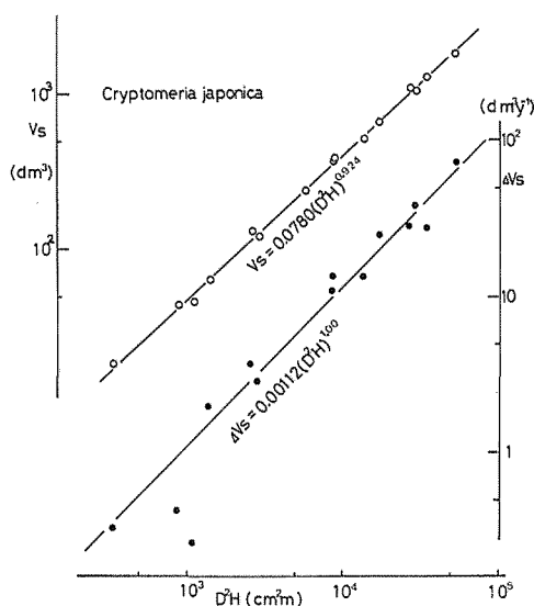
Fig. 4 Relations of stem volume ( V_s ) and stem volume increment ( \Delta V_s ) to D^2H .
