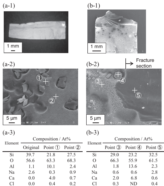
Figure 5. (a-1) A microscope image, (a-2) SEM image, and (a-3) EDX analysis result for a borosilicate glass plate soaked in molten \text{CaCl}_2 for 30 min at 1123 K and rinsed in distilled water. SEM images in (b-1) low and (b-2) high magnification, and (b-3) EDX analysis result from a fractured surface obtained by breaking the plate after immersion shown in (a-1).
