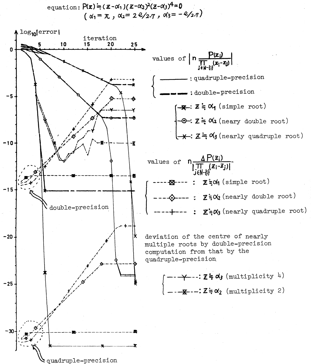
Fig. 9. Comparison of the resolution powers of computation of different precisions when there are clusters of zeros located very close to one another
