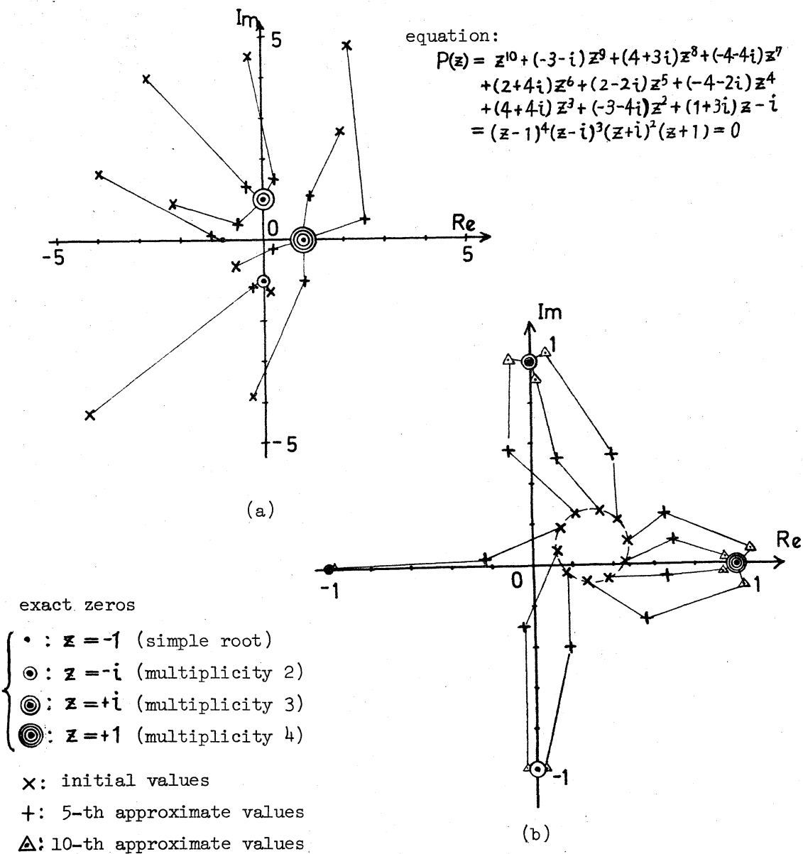
Fig. 4. Trajectories of the approximate points from different initial points
