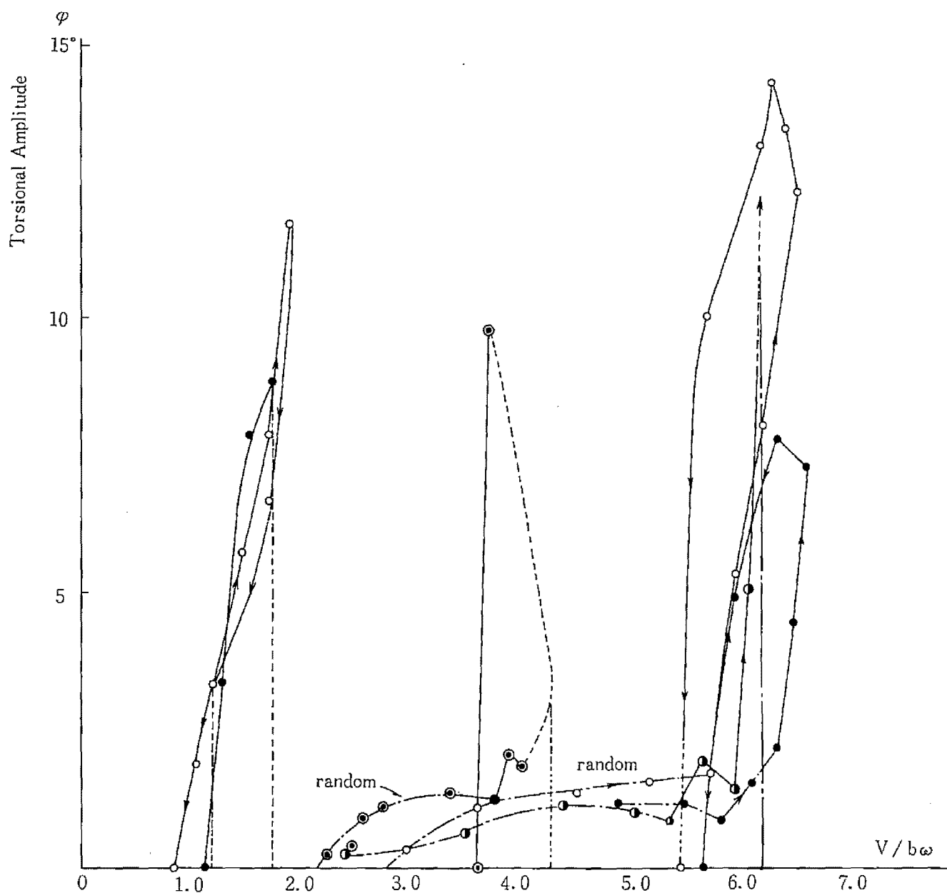
Fig. 4.24 Response-Reduced Velocity Relation in Turbulent Flow
