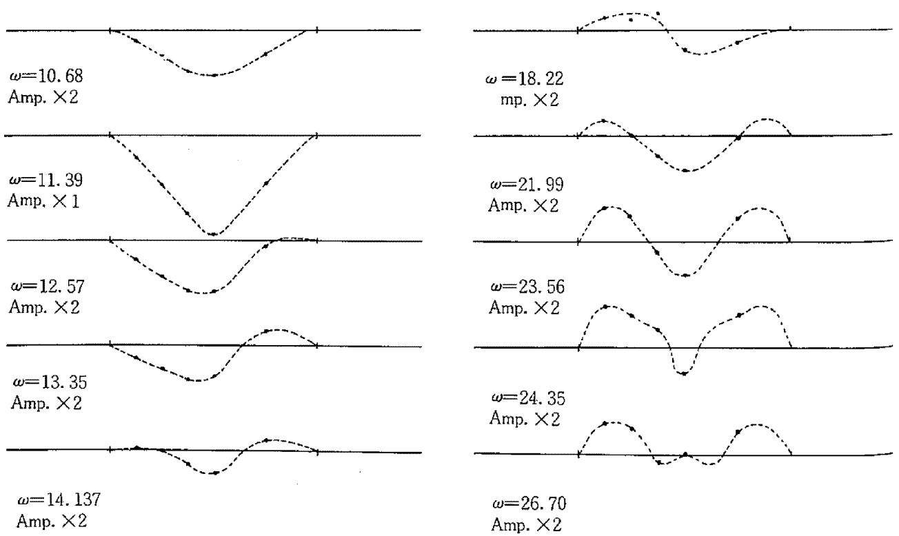
Fig. 2.33 Forced Vibration Test for Double Warren Type Hanger System (Forced at midpoint of Main Span)
