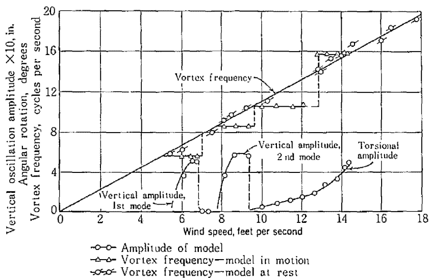
Vortex frequency vs. wind speed .
