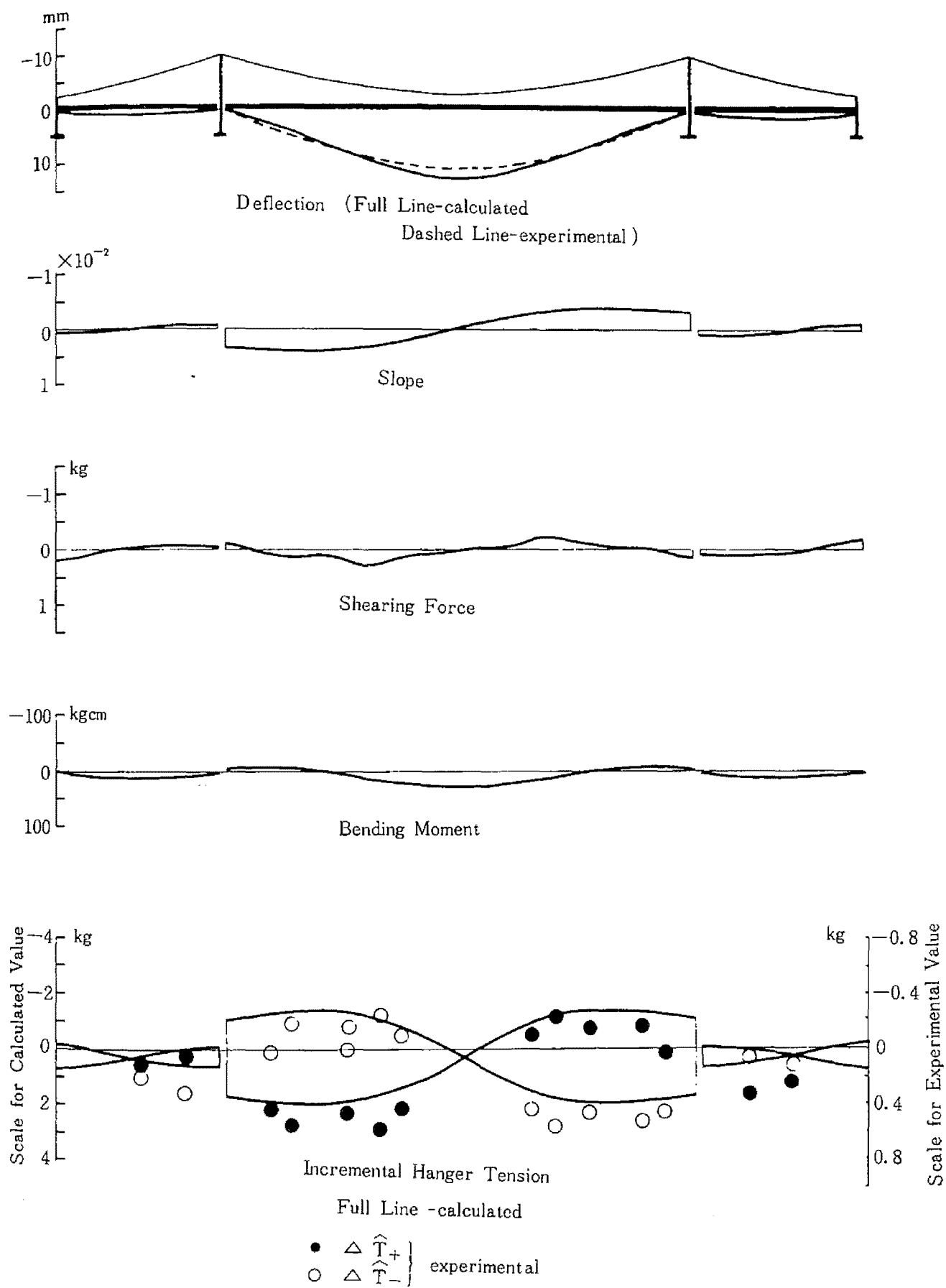
Fig. 2.24 Inclined Hanger System(Fully Loaded)
