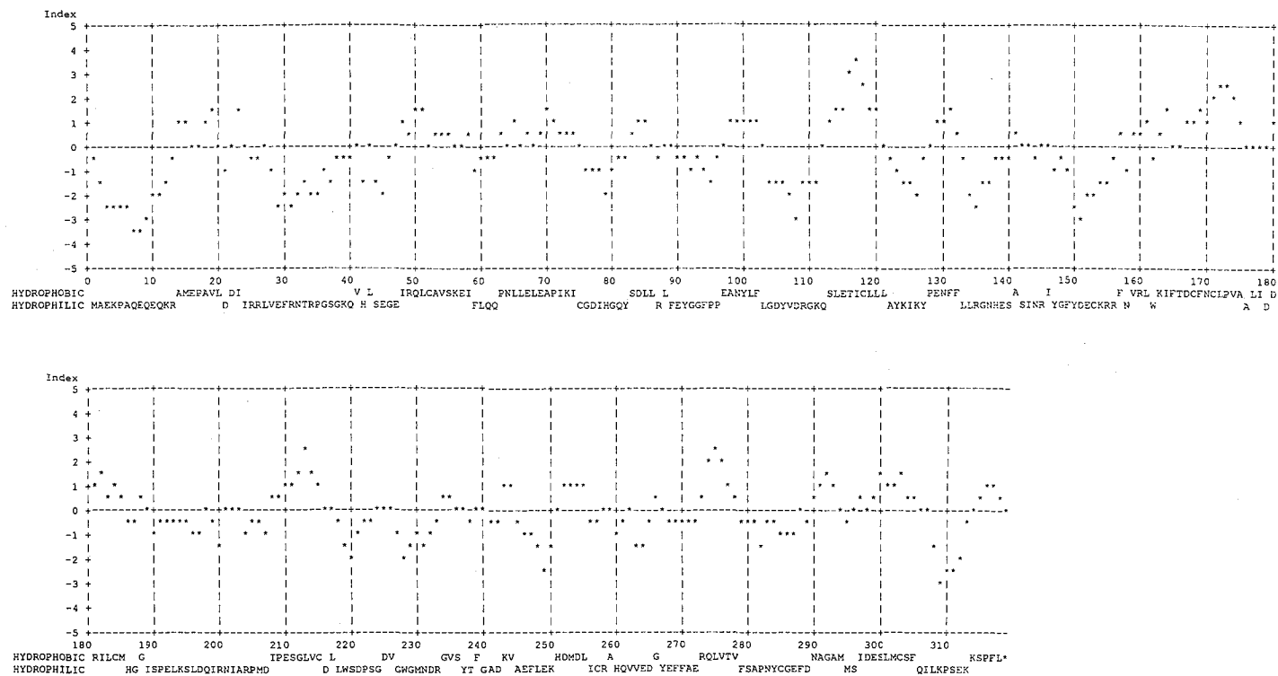
Fig. 3. Hydropathy profile of AT-PP1. Positive and negative values indicate hydrophobic and hydrophilic characters, respectively. 27)
