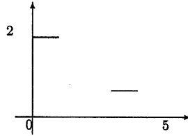
FIGURE 2. A walk in \Omega_{10}^5 with two successive Null steps from (0, 3) to (0, 3) .
