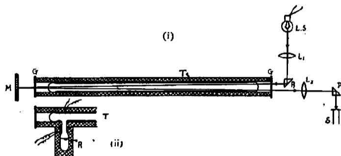
Fig. 2. Experimental apparatus for photographing the absorption spectrum of the vibration-rotation bands of water vapour.
