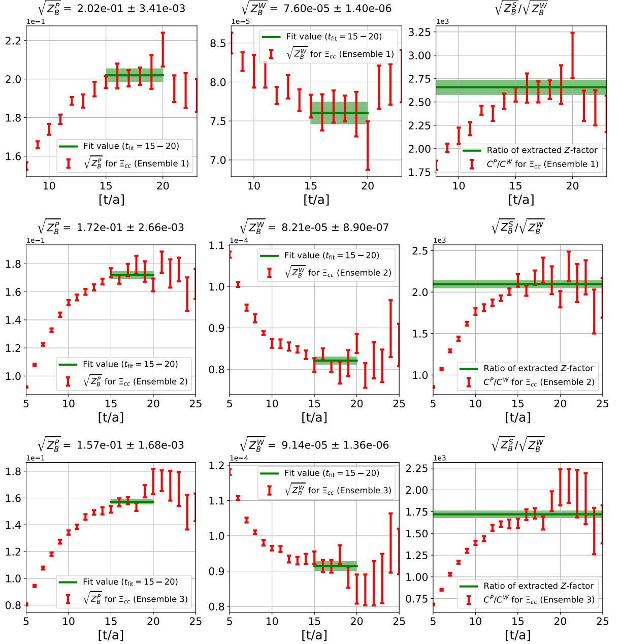
Figure C.4: The fitting results of the Z -factors for \Xi_{cc} . Upper three figures correspond to the results for the ensemble 1 ( m_\pi \simeq 700 MeV case). Middle three figures correspond to the results for the ensemble 2 ( m_\pi \simeq 570 MeV case). Lower three figures correspond to the results for the ensemble 3 ( m_\pi \simeq 410 MeV case).
