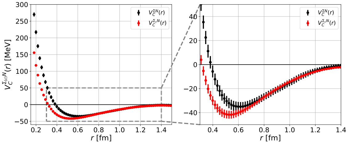
Figure 5.14: The comparison between the central potential for the \Sigma_c N channel and the \Sigma N channel in the ^3S_1 channel. The potentials are calculated at t - t_0 = 13 for m_\pi \simeq 700 MeV case.
