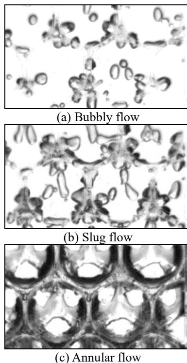
Figure 3 Two-phase flow patterns
