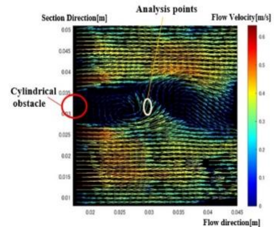
Fig. 2. PIV result photographed a wake of cylinder(6.3 mm diameter).
