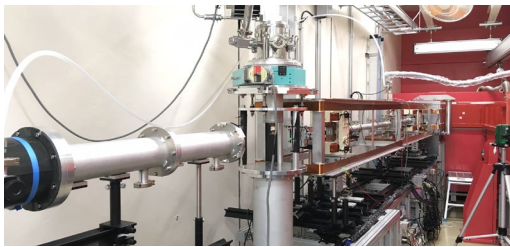
Fig. 1. The MIEZE-type neutron spin echo spectrometer of VIN ROSE at BL06 at J-PARC MLF.
