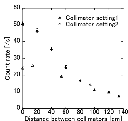
Fig. 3. Dependence of distance between collimators and ^{10}\text{B} count rate.
