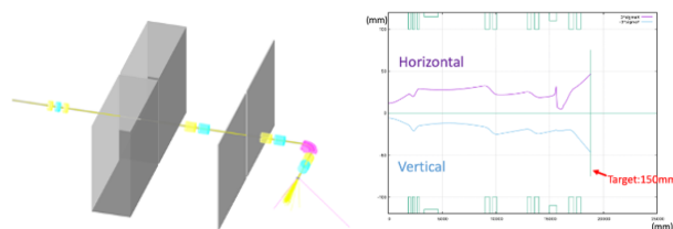
Fig. 2. Simulation of the new beam transport for accelerator driven neutron source using G4beamline (left). Beam tracking result of the second beam transport (BT2) for accelerator driven neutron source using G4beamline (right).
