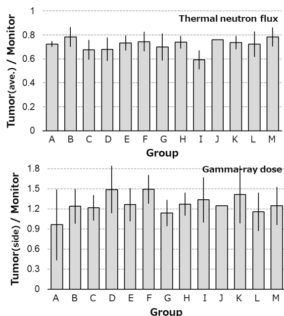
Fig. 2. Average tumor/monitor ratios by each research group.
