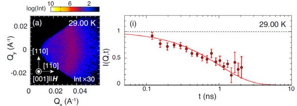
Fig. 3. Neutron scattering data of Skyrmion phase of MnSi just above the critical temperature. (Left) The diffuse scattering pattern on the Q_x - Q_y plane. (Right) I(Q, t) curve fitted by a single exponential function with time constant \tau = 1.02(5) ns [4].
