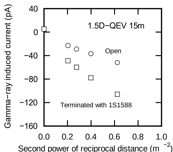
Fig. 1. Dependence of the gamma-ray induced current of coaxial cable on the second power of the reciprocal distance from the gamma-ray source.
