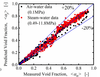
Fig.2 Comparison between experimental and predicted data
