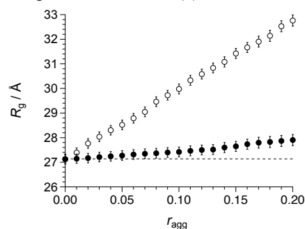
Fig. 2. Weight fraction of aggregates r_{agg} dependences of gyration radii R_g derived from the non-treated scattering profiles (white circles) and AUC-SAS treated scattering profiles (black circles).
