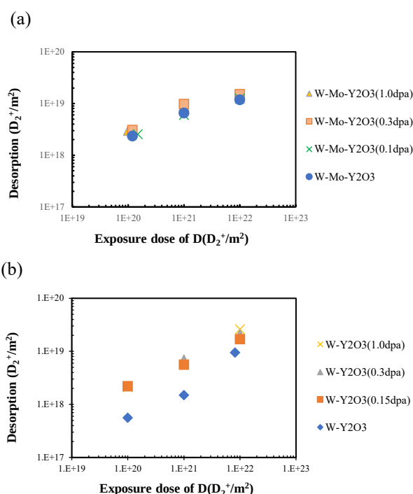
Fig.1 Relationship between the D 2 desorption and D 2 irradiation dose in W-Mo-Y 2 O 3 (a) and W-Y 2 O 3 (b) alloys.
