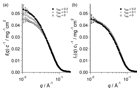
Fig. 1. (a) Calculated scattering profiles for the BSA including aggregation at r_{agg} = 0 (white), 0.1 (gray), and 0.2 (black). (b) AUC-SAS-treated scattering profiles for the profiles shown in (a).
