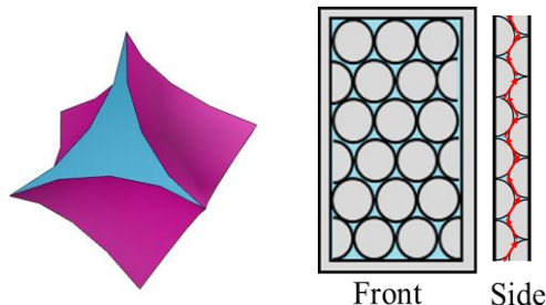
Figure 1 Minimal flow channel unit
