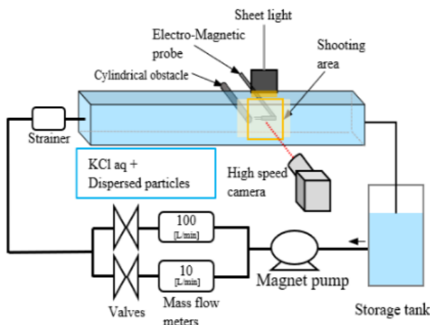
Fig. 1. Experimental setup.
