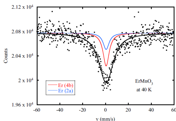
Fig. 5. ^{166}\text{Er} Mössbauer spectra of \text{ErMnO}_3 [8]
