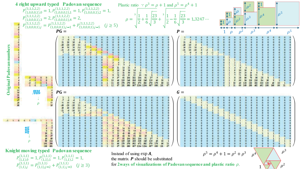
Figure 16 2 ways of visualizations for Padovan sequence and plastic ratio on modified Pascal's triangles.
