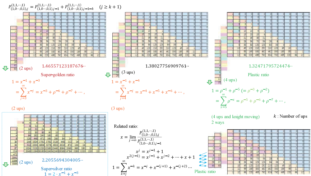
Figure 10 Illustrative examples of 2, 3, and 4 upward typed sequences on related Pascal's triangles and these ratios.
