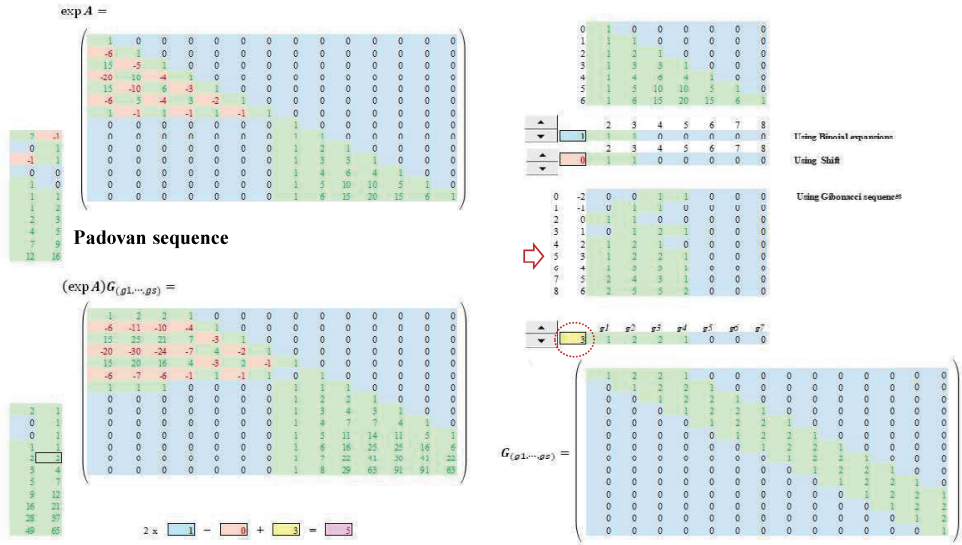
Figure 8 Illustrative examples for changing the initial conditions of Padovan sequence applying band matrices G .
