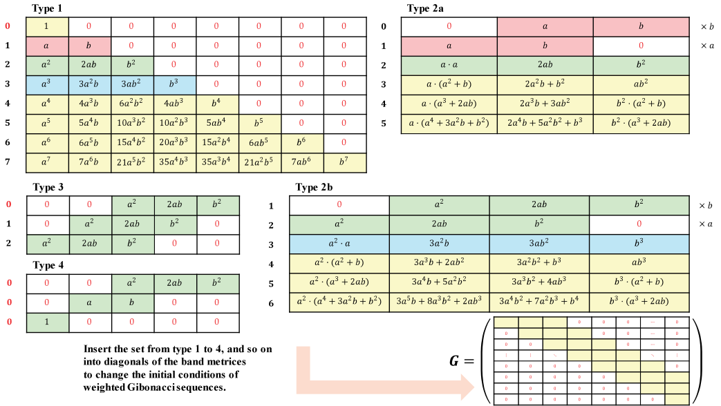
Figure 3 Illustrative examples for changing initial conditions to move smoothly using band matrices G .
