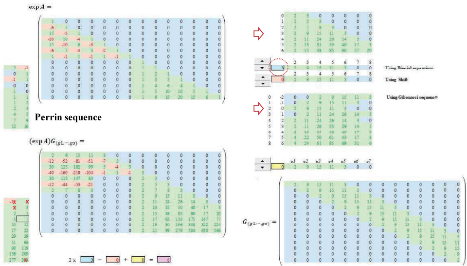
Figure 9 Illustrative examples for changing the initial conditions of Perrin sequence applying band matrices \mathbf{G} .
