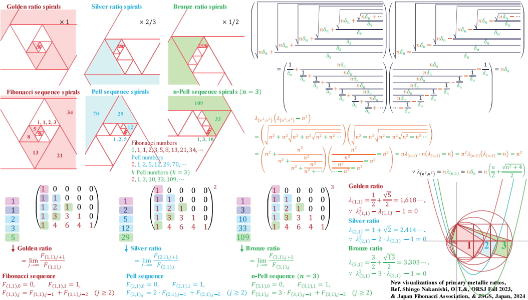
Figure 14 Illustrative examples for double spirals of equilateral triangles as golden ratio, silver ratio, bronze ratio of primary metallic ratios and these characterizations on modified Pascal's triangles [32,33,35].
