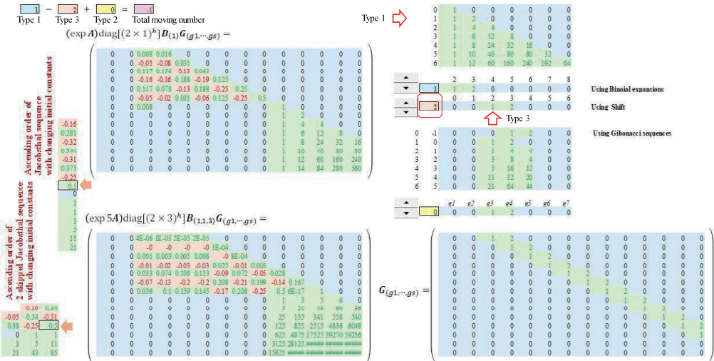
Changing initial conditions smoothly (-1 moved condition)
