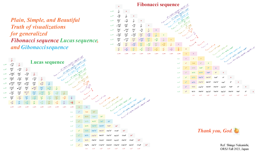
Figure 17 Artistic Illustrative examples for weighted Fibonacci sequence and Lucas sequence on modified Pascal's triangles [9,37].
