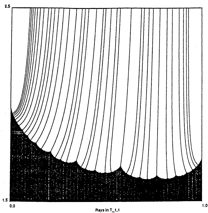
Figure III. The real trace lines.
