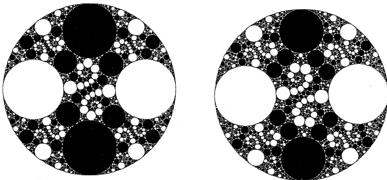
Figure II. Limit sets of cusp groups. The two different circle packings correspond to pinching different pairs of curves.
