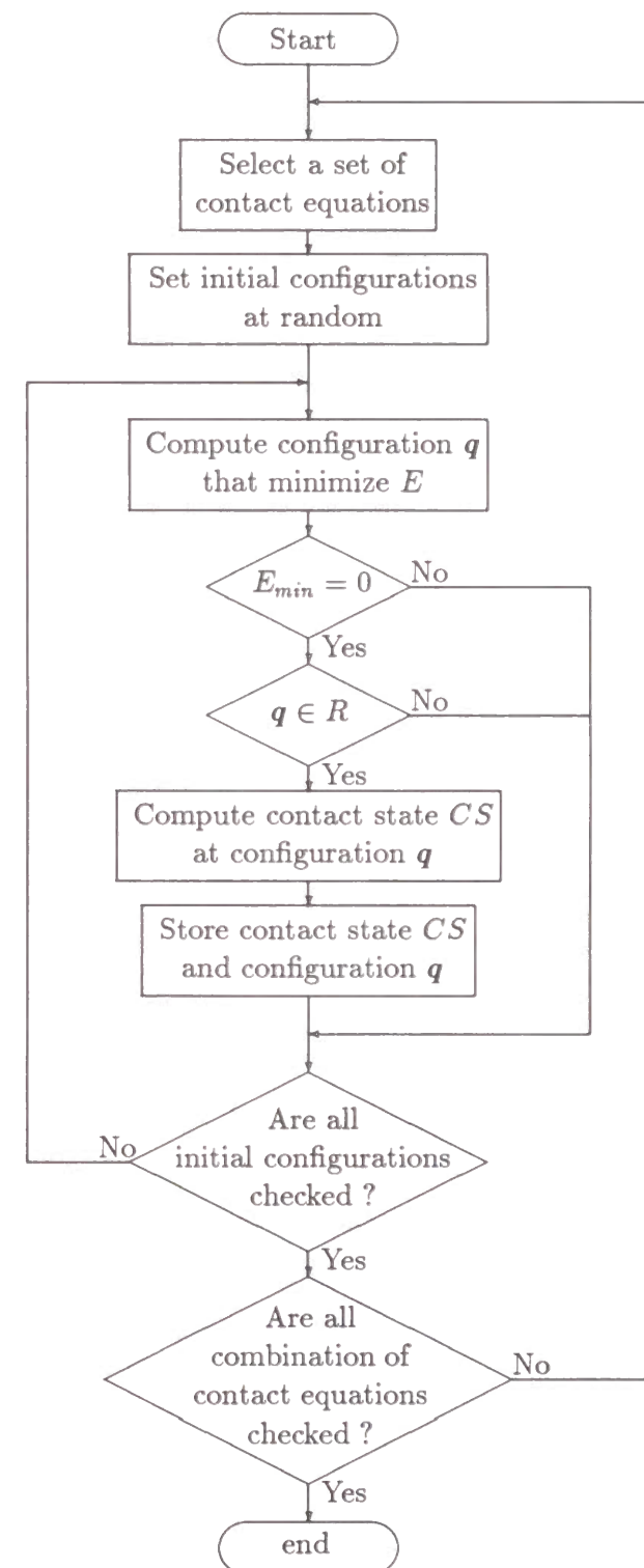
Figure 13: Algorithm to obtain sample configurations
