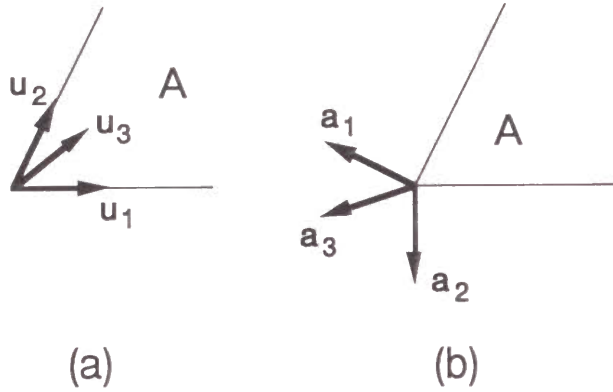
Figure 9: Simplification of polyhedral convex cones
