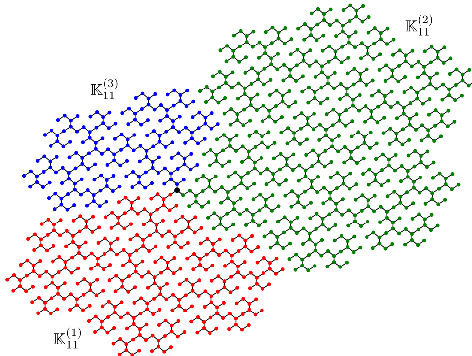
Figure 4. The set \mathbb{P}_{11} . In order to enlight the tree structure the point \mathbf{0} is shown in black and adjacent points are connected.
