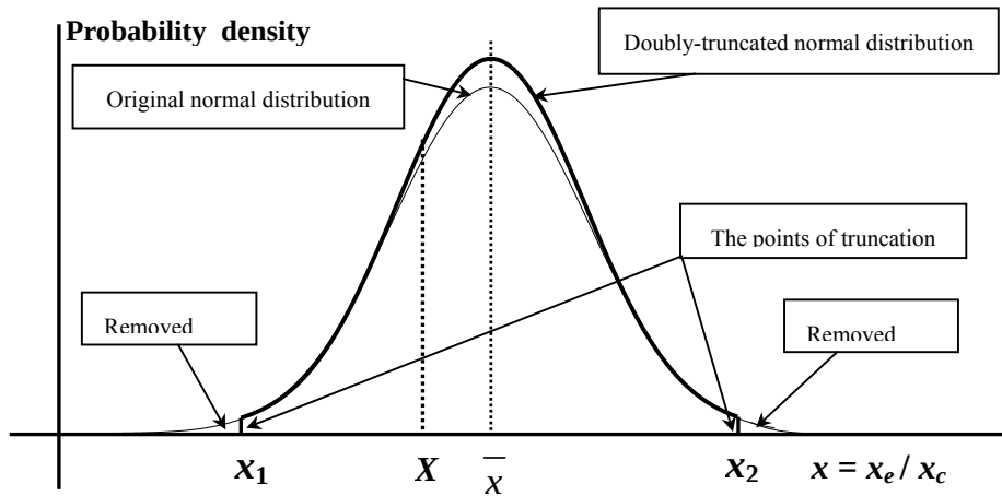
Fig. 9 Conceptual explanation of a doubly-truncated normal distribution
