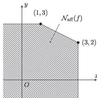
図 2: Affine Newton polyhedron \mathcal{N}_{\text{aff}}(f)
