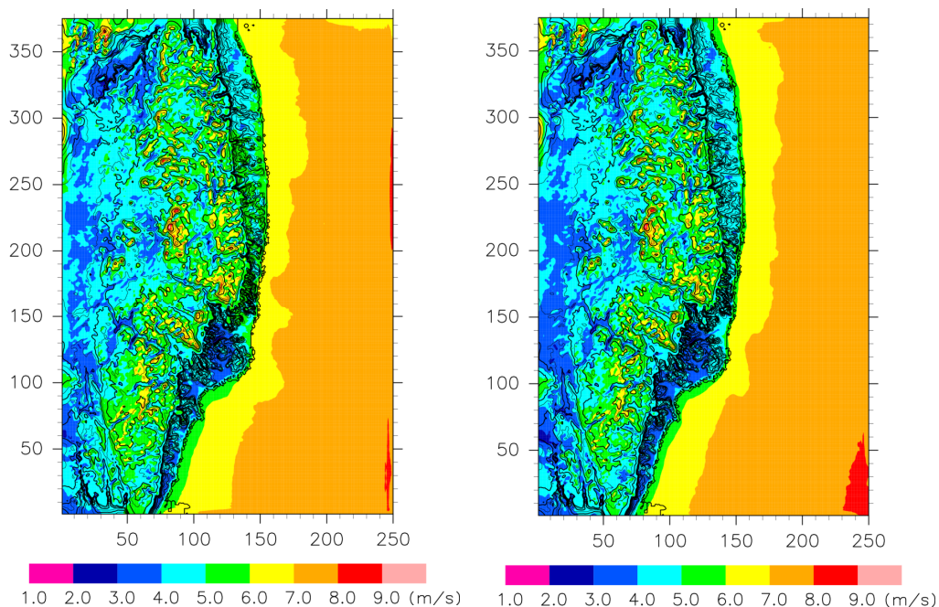
Fig. 3 Spatial distribution of 10-m-level wind speed average in time during the simulated period for the MYJ case (left) and the QNSE case (right) in Domain 3. The solid contour lines indicate the surface elevation.
