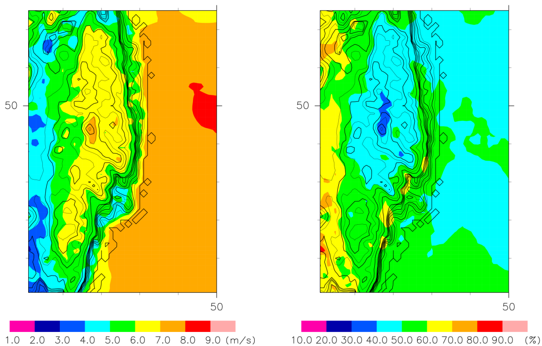
Fig. 6 The same as Fig. 5, except for the case obtained in Domain 2. The area corresponds to the Domain 3 is chosen from the total area of Domain 2.
