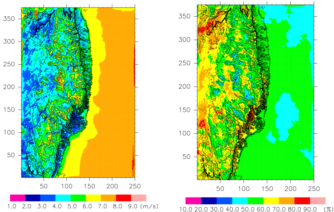
Fig. 5 Spatial distribution of surface wind speed average in time (left) and its standard deviation normalized by the averaged wind speed (right) for the MYJ case in Domain 3. The surface wind here refers to the wind at the 10-m height AGL. The solid contour lines indicate the surface elevation.
