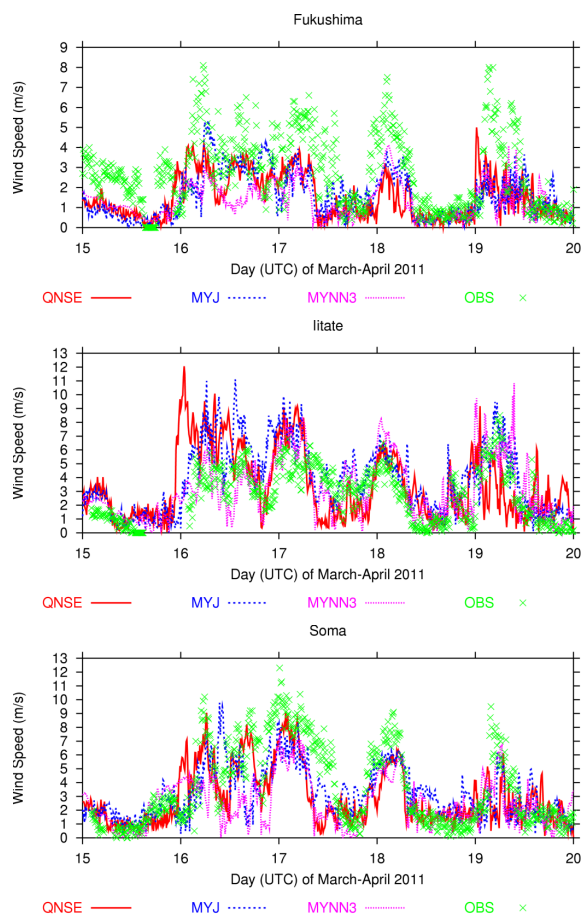
Fig. 2 Time series of surface wind speed from observation (green) and from numerical simulations with the MYJ (blue), the QNSE (red), and the MYNN3 (pink) scheme at Fukushima City (upper), Iitate Town (middle), and Soma City (lower).
