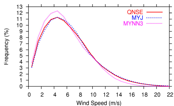
Fig. 4 Frequency distribution of wind speed at the 10-m height above the ground level (AGL) for the QNSE (red), the MYJ (blue), and the MYNN3 (pink) case in Domain 3.
