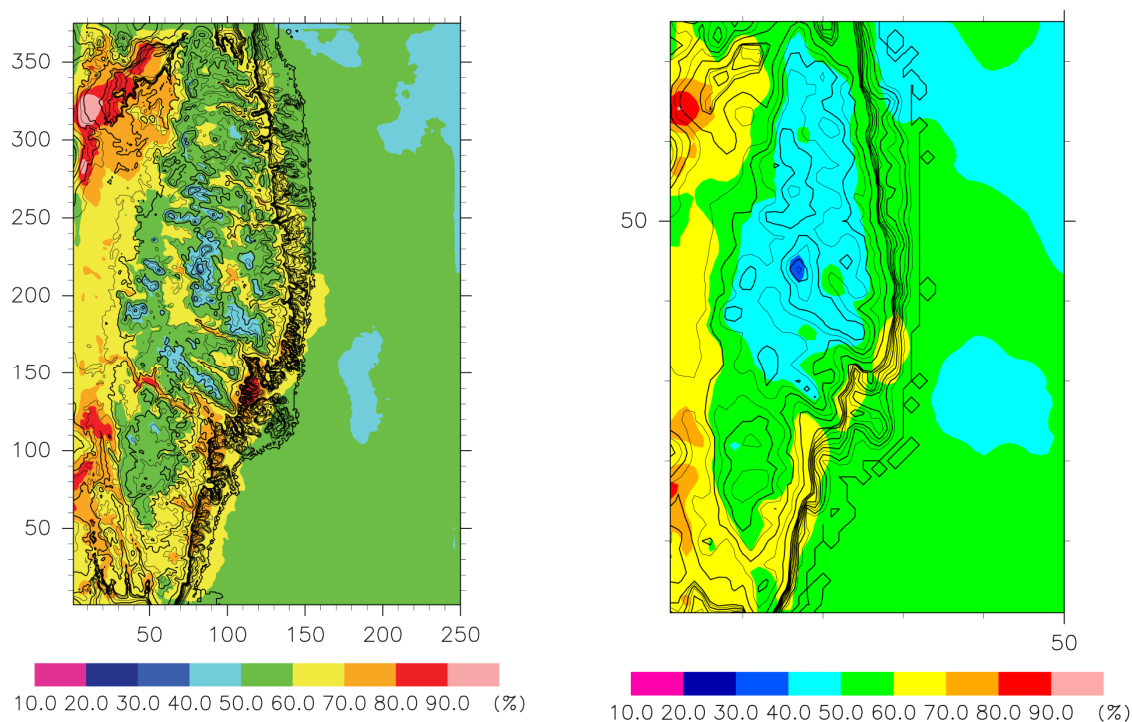
Fig. 7 Spatial distribution of the normalized standard deviation of wind speed at the 100-m AGL for the MYJ case in Domain 3 (left) and Domain 2 (right). The solid contour lines indicate the surface elevation.
