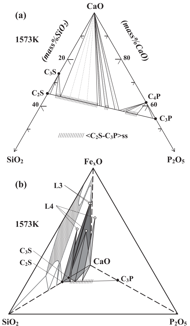
Fig. 2. (a) Iso-thermal section of the \text{CaO-SiO}_2\text{-P}_2\text{O}_5 ternary system at 1 573 K. 9) (b) Schematic diagram of phase relationship in the \text{CaO-SiO}_2\text{-P}_2\text{O}_5\text{-Fe}_x\text{O} quaternary system at 1 573 K.
