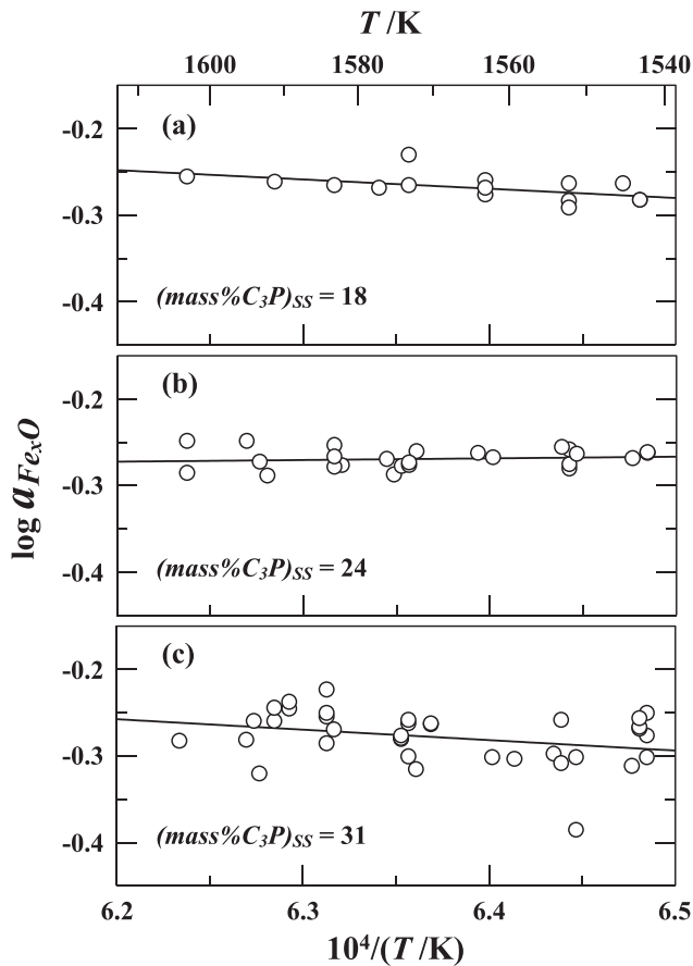
Fig. 8. Relation between logarithmic value for \text{Fe}_x\text{O} activity and reciprocal temperature.
