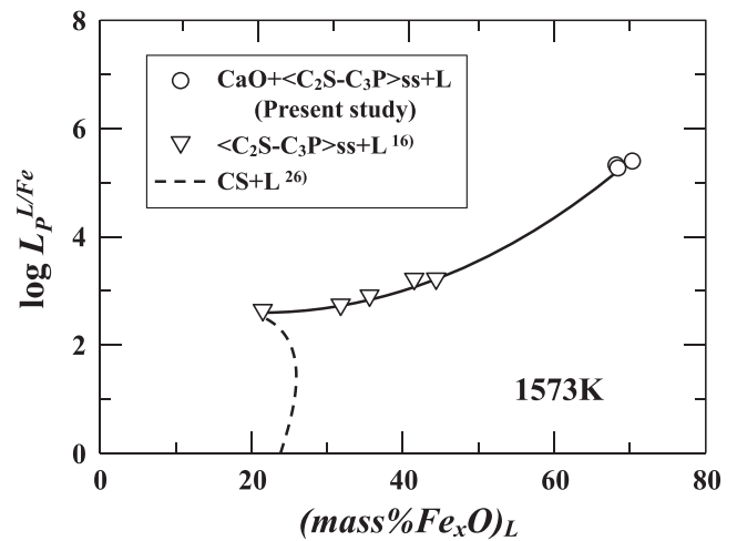
Fig. 10. Phosphorus distribution ratio between liquid slag and molten iron plotted against \text{Fe}_x\text{O} content in liquid slag.
