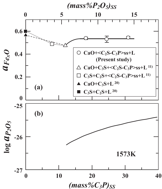
Fig. 9. Relation between the activity and the \text{C}_3\text{P} content in \text{C}_2\text{S} – \text{C}_3\text{P} solid solution at 1573 K. (a) \text{Fe}_x\text{O} , (b) \text{P}_2\text{O}_5 .
