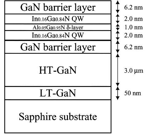
Fig. 1. Schematic layer structure of the sample with the AlGaIn \delta -layer grown by MOVPE.
