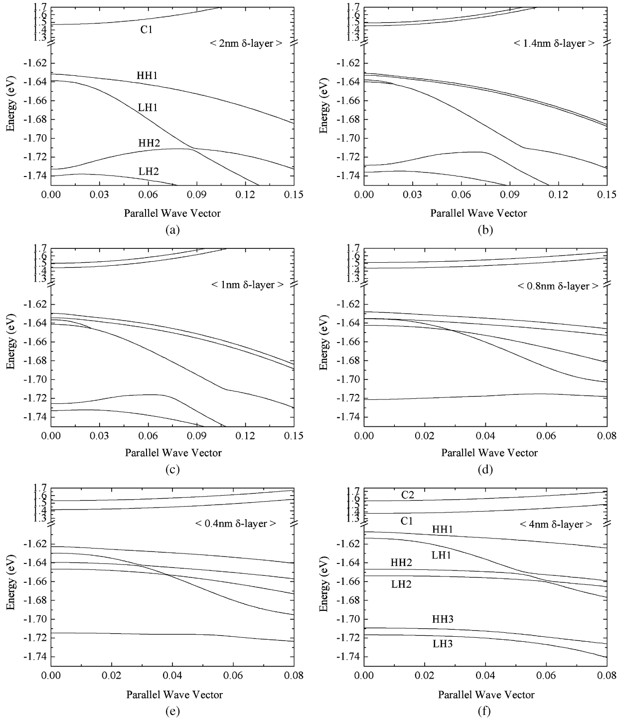
Fig. 4. In-plane dispersion of conduction and valence subbands of 2-nm-thick \text{In}_{0.16}\text{Ga}_{0.84}\text{N} SQW, \text{In}_{0.16}\text{Ga}_{0.84}\text{N} QWs with 0.4-, 0.8-, 1.0-, and 1.4-nm-thick \text{Al}_{0.05}\text{Ga}_{0.95}\text{N} \delta -layers, and 4-nm-thick \text{In}_{0.16}\text{Ga}_{0.84}\text{N} SQW.
