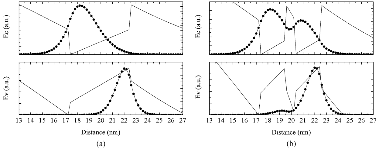
Fig. 7. Energy band diagram and wave function of (a) 5-nm-thick \text{In}_{0.16}\text{Ga}_{0.84}\text{N} SQW and (b) \text{In}_{0.16}\text{Ga}_{0.84}\text{N} (2 nm) – \text{Al}_{0.05}\text{Ga}_{0.95}\text{N} (1 nm \delta – layer) – \text{In}_{0.16}\text{Ga}_{0.84}\text{N} (2 nm) QW sandwiched between 10-nm-thick GaN barriers at zero bias current.
