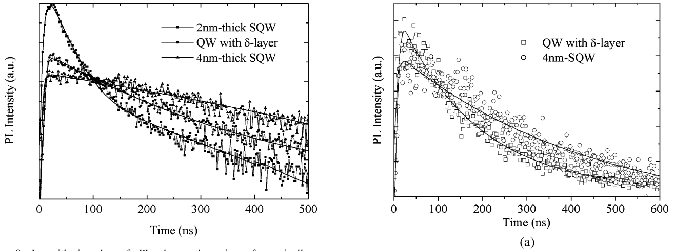
Fig. 8. Logarithmic plot of PL decay dynamics of nominally undoped 2-nm-thick \text{In}_{0.16}\text{Ga}_{0.84}\text{N} SQW, \text{In}_{0.16}\text{Ga}_{0.84}\text{N} (2 nm) – \text{Al}_{0.05}\text{Ga}_{0.95}\text{N} (1 nm) – \text{In}_{0.16}\text{Ga}_{0.84}\text{N} (2 nm) QW, and 4-nm-thick \text{In}_{0.16}\text{Ga}_{0.84}\text{N} SQW.
