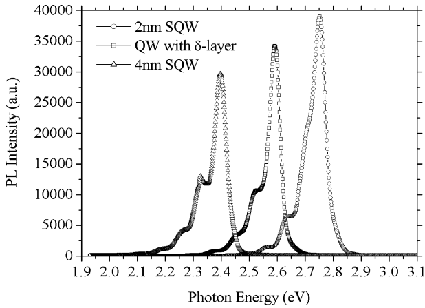
Fig. 5. Low-temperature (13 K) continuous-wave PL spectra of nominally undoped 4-nm-thick \text{In}_{0.16}\text{Ga}_{0.84}\text{N} SQW ( -\triangle- ), \text{In}_{0.16}\text{Ga}_{0.84}\text{N} (2 nm) – \text{Al}_{0.05}\text{Ga}_{0.95}\text{N} (1 nm)– \text{In}_{0.16}\text{Ga}_{0.84}\text{N} (2 nm) QW ( -\square- ), and 2-nm-thick \text{In}_{0.16}\text{Ga}_{0.84}\text{N} SQW ( -\circ- ).
